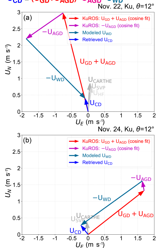
Figure 16. Comparison of KuROS-derived Doppler velocity, corrected for the U_{\text{AGD}} and U_{\text{WD}} wave contributions, with in situ (CARTHE, SVP drifters and HF radar) current measurements on (a) 22 and (b) 24 November.
