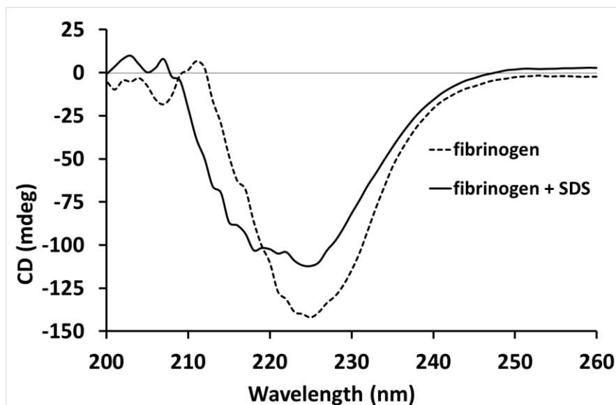
Figure SI-2: CD spectra of fibrinogen in saline solution at 37°C without (---) or with (—) Sodium Dodecyl Sulfate (50 mM).
