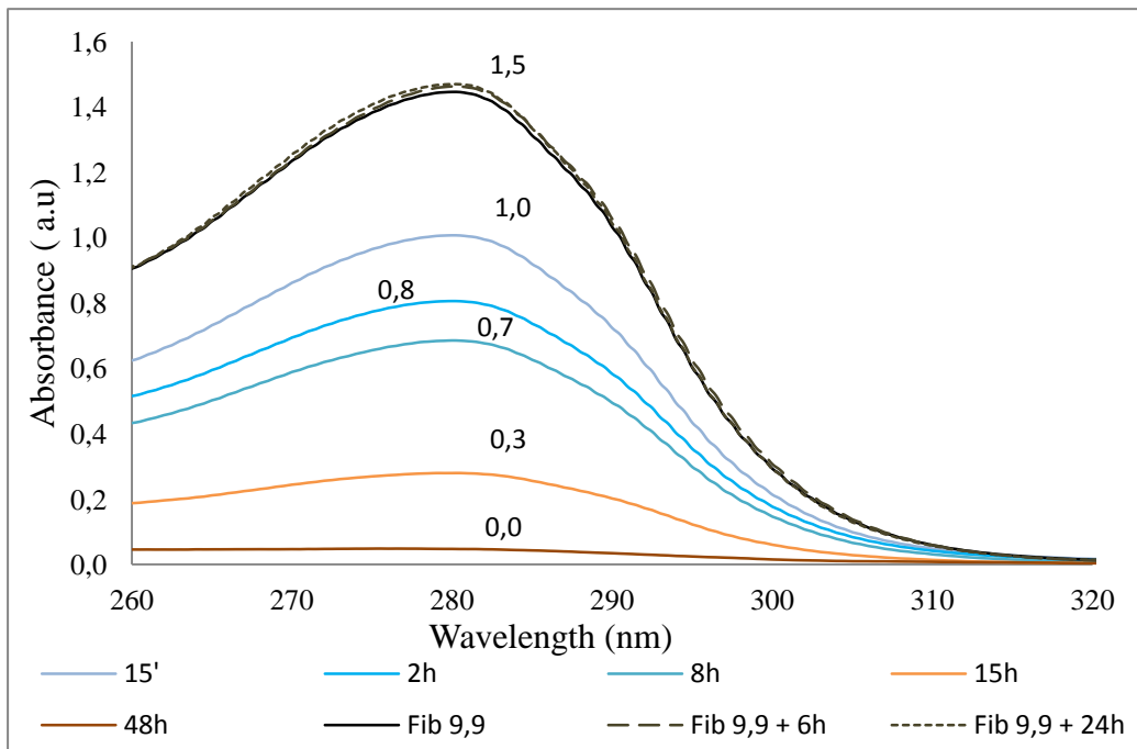
Figure SI-1: Evolution of absorbance spectra of supernatant solution as a function of 92 S6 P123 glass soaking time: 15 min (1.0), 2h (0.8), 8h (0.7), 15h (0.3) and 48 h (0.0). The absorbance spectra of fibrinogen solution at the same pH that the supernatant solution (9,9) at different times: 0, 6 h and 24 h are also presented (1,5).
