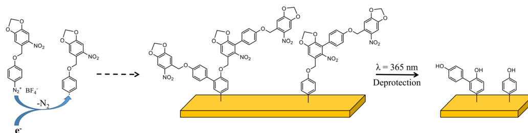
Scheme 1 Schematic representation of aryl diazonium 1 and of the grafting process and the resulting organic deposit after deprotection.
