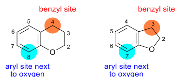
Figure 2. Similarities between chromane (left) and 2,3-dihydrobenzofuran (right).
