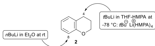
Figure 10. Bases already employed to functionalise chromane ( 2 ).
