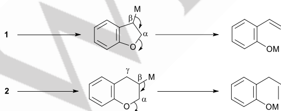
Figure 8. Possible side-processes. M = alkali metal.
