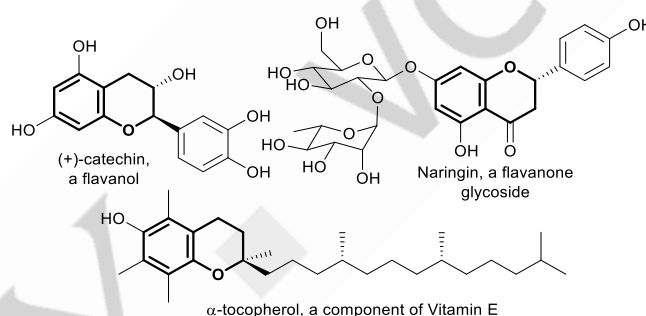
Figure 1. Structures of a few bioactive chromane-based compounds.
