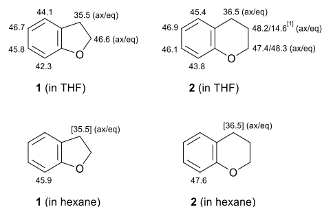
Figure 6. pK_a values calculated for 2,3-dihydrobenzofuran ( 1 ) and chromane ( 2 ) in THF (top) and hexane (bottom). As references with known pK_a values in hexane were not available, we arbitrarily set the ones for the benzyl position (in square brackets) at C3 (compound 1 ) and C4 ( 2 ) as those calculated in THF. [1] Ring opening expected.
