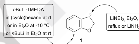
Figure 9. Bases already employed to functionalise 2,3-dihydrobenzofuran ( 1 ).
