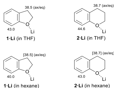
Figure 7. pK_a values calculated for the complexes of 2,3-dihydrobenzofuran ( 1 ) or chromane ( 2 ) with either \text{LiNMe}_2 \cdot 2\text{THF} in THF (top) or \text{MeLi} \cdot \text{TMEDA} in hexane (bottom). As references with known pK_a values in hexane were not available, we arbitrarily set the ones for the benzyl position (in square brackets) at C3 (compound 1 ) and C4 ( 2 ) as those calculated in THF.
