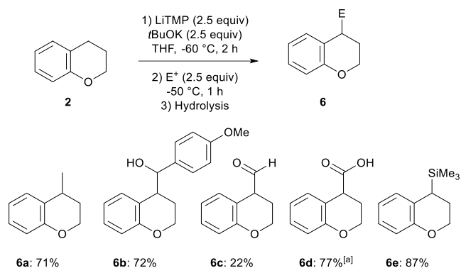
Scheme 1. Functionalisation of chromane ( 2 ) at C4 by deprotonation-trapping using different electrophiles. [a] Isolated as a tautomeric form.
