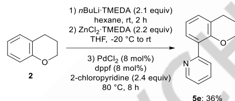
Scheme 3. Functionalisation of chromane ( 2 ) at C8 by deprotonation, transmetalation to zinc and Negishi coupling.
