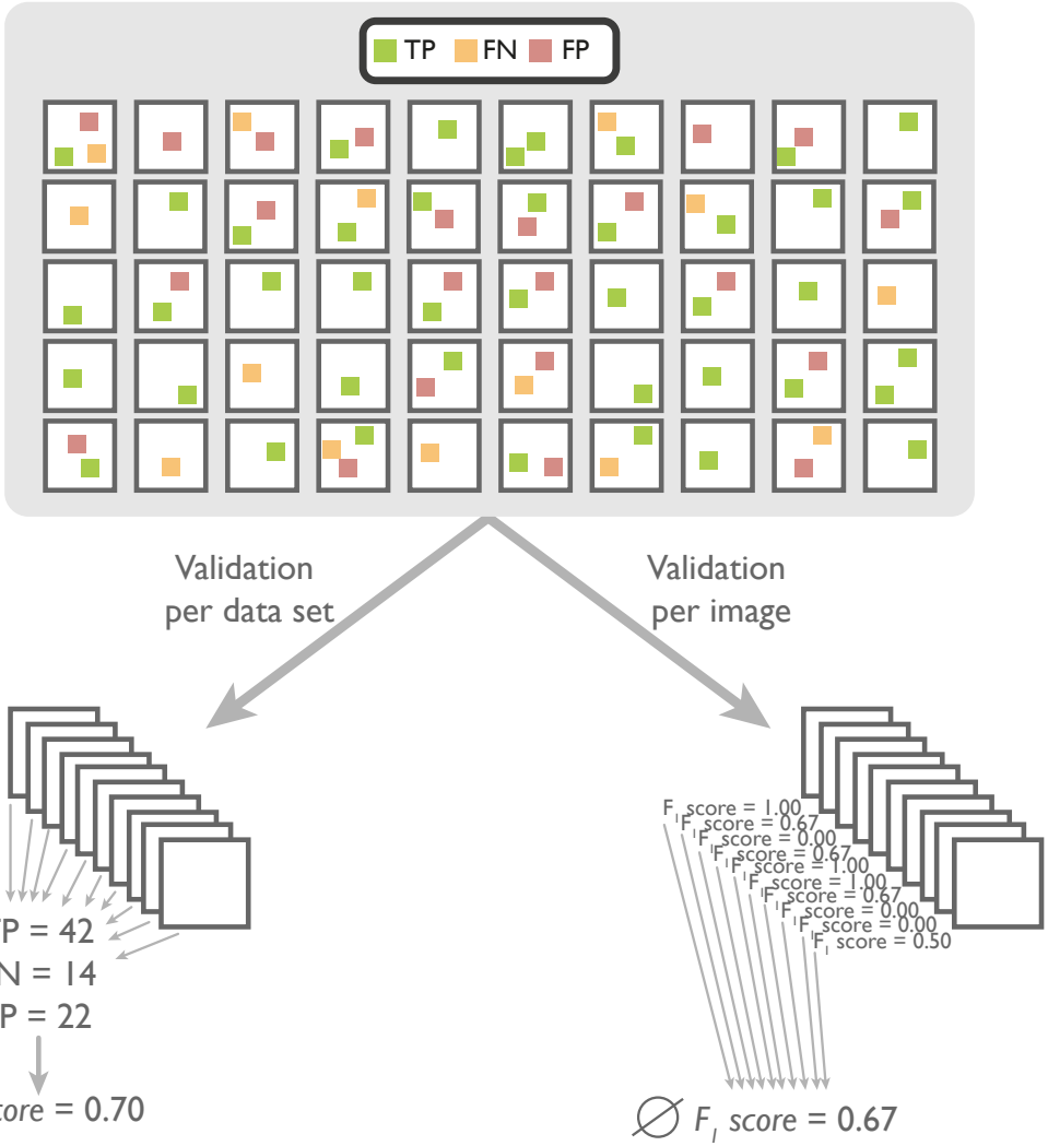
Extended Data Fig. SN 2.10. Validation on object level can be performed per data set (left) or per image (right). For the per-data set validation of objects, the cardinalities are calculated over the whole data set. For the per-image validation of objects, metric scores are computed per image and aggregated afterward. \emptyset refers to the average F_1 Score.
