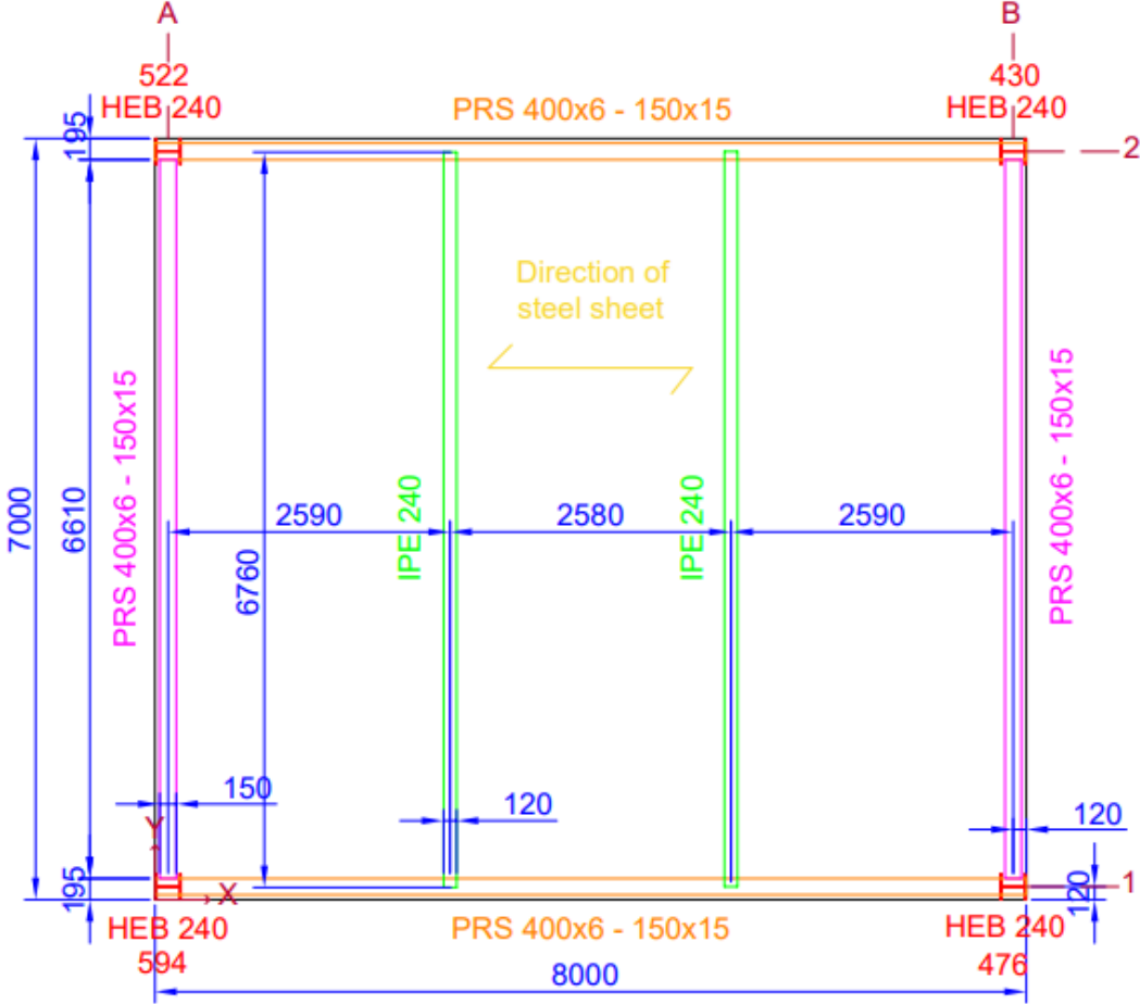
(a) Plan view (columns heights in red)
