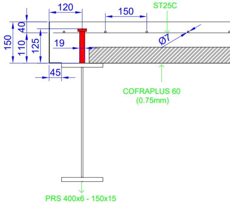
(b) Front view (steel sheet in grey, shear stud in red)
