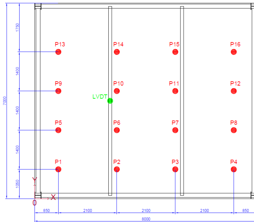
(b) Positions of individuals (red circles) and LVDT (green circle) Figure 5: Crowd-rhythmic test setup (dimensions in mm)
