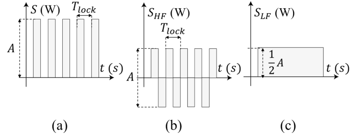
Fig. 3. Modulation signal: (a) S(t) , (b) S_{HF}(t) , (c) S_{LF} .
