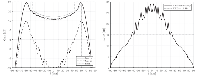
(c) Radiation in cut \phi = 90^\circ .
