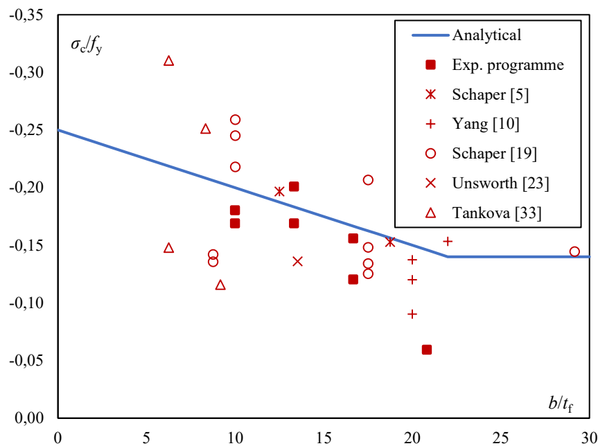
Figure 11: Flanges compressive stresses: Experimental and analytical results
