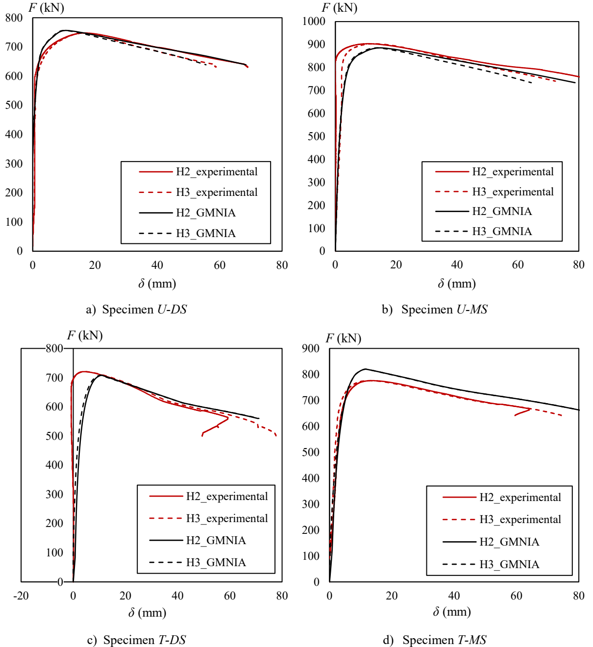
Figure 28: Force–global displacement curves: Experimental and numerical results
