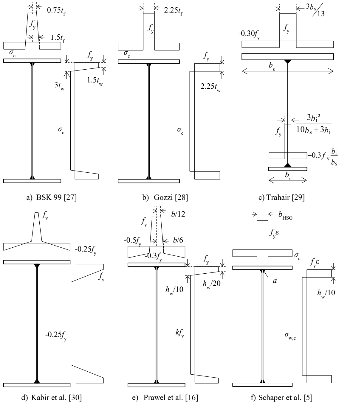
Figure 2: Residual stress models for welded members made of hot-rolled flanges
