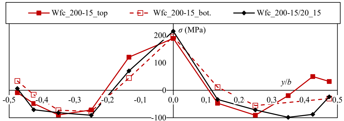
Figure 8: Residual stresses in 200x15-mm flame-cut flanges
