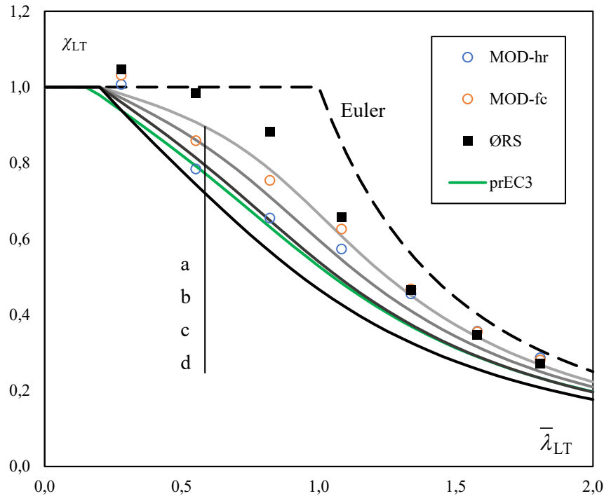
Figure 30: Numerical results for U-DS under a constant bending moment
