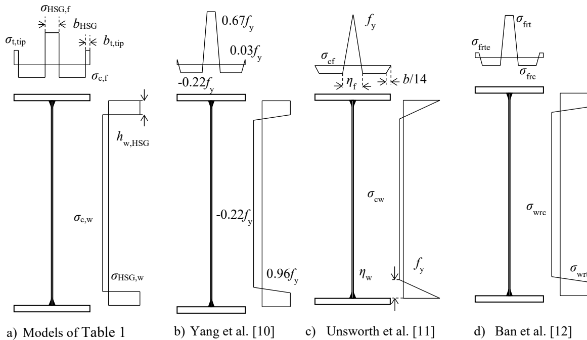
Figure 3: Residual stress models for welded members made of flame-cut flanges
