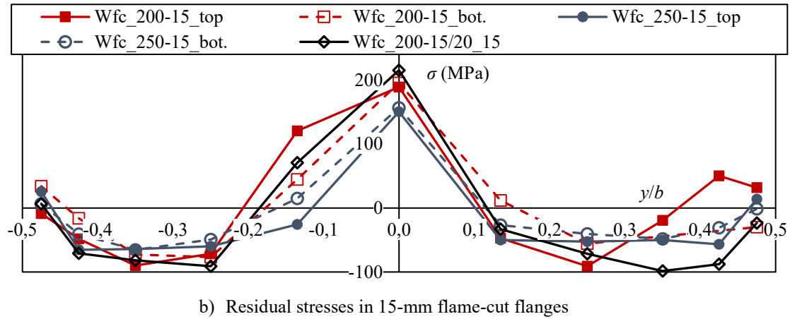
Figure 6: Residual stresses in flame-cut flanges with varying width
