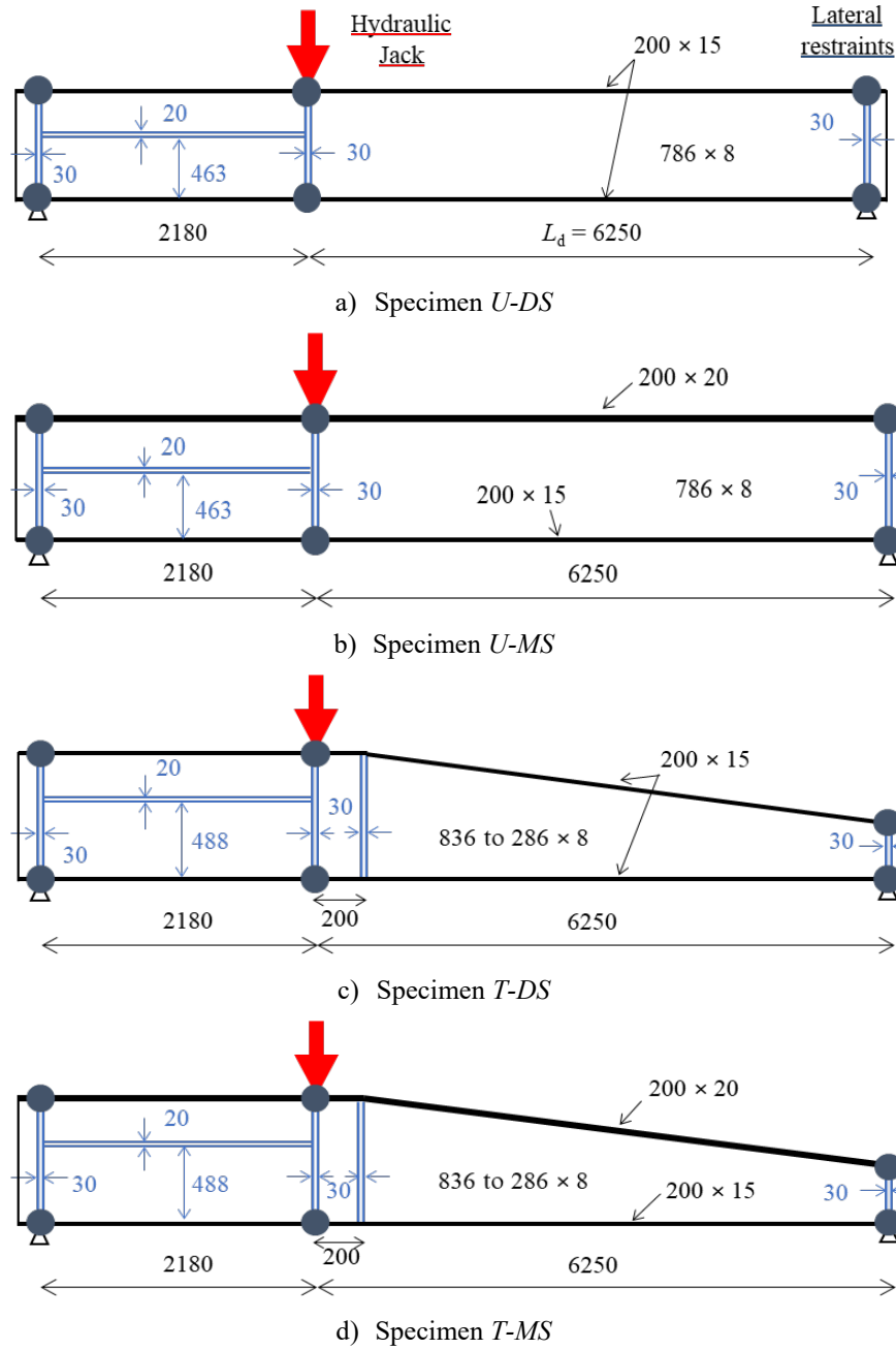
Figure 14: Test specimens (dimensions in mm)
