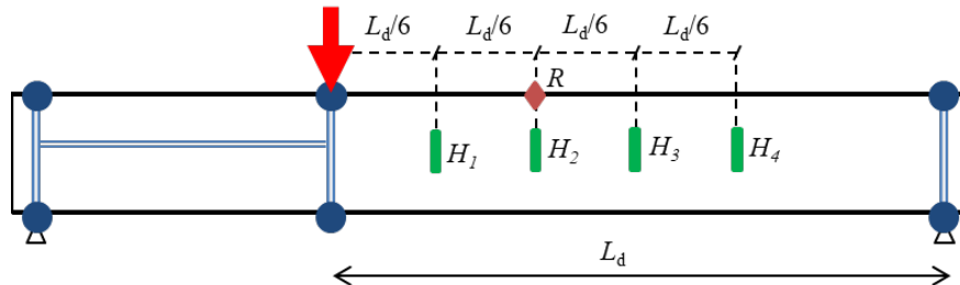
Figure 15: Global displacement and twist rotation measurements
