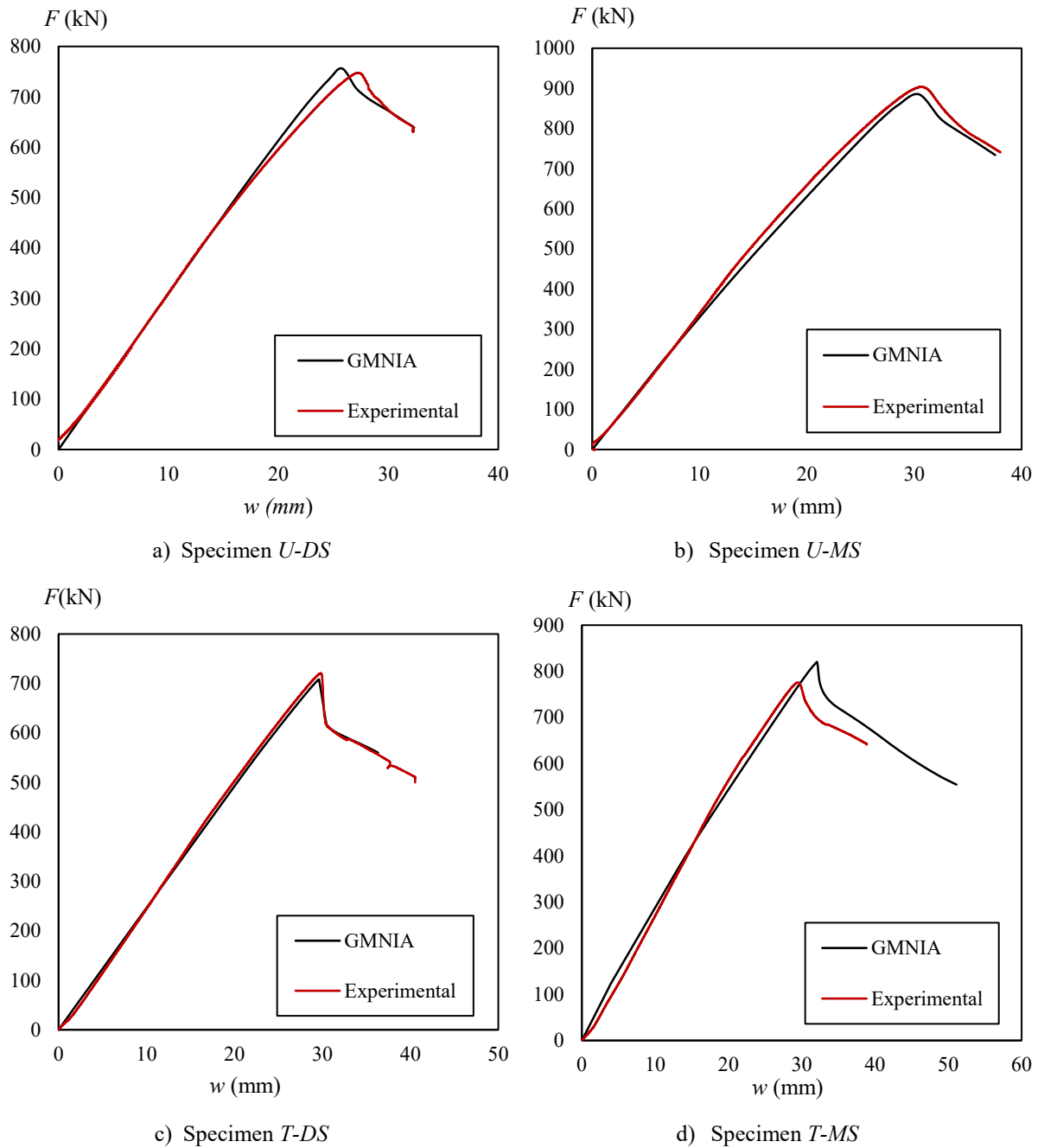
Figure 27: Force–vertical displacement curves: Experimental and numerical results
