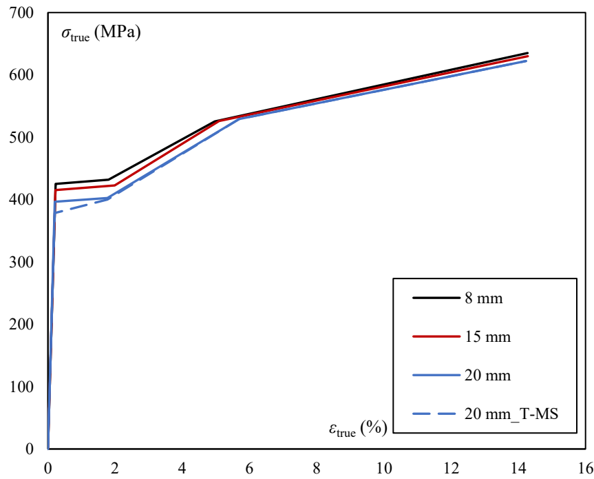
Figure 24: Stress-strain curves used in the FE analyses
