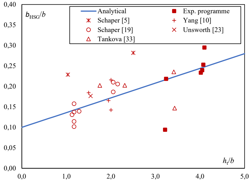
Figure 13: Width of the flange central tension region: Experimental and analytical results
