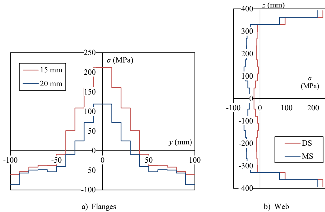
Figure 29: Residual stresses used in the FE analyses for welded beams made of hot-rolled flanges
