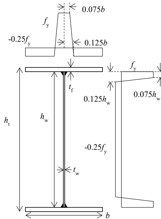
Figure 1: Residual stress model of prEN 1993-1-14 [25] (hot-rolled flanges)
