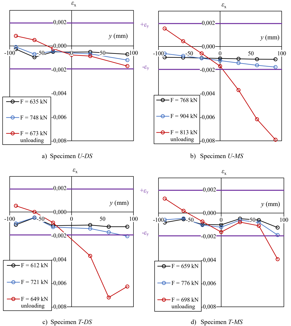
Figure 23: Axial strains in compression flanges of the critical cross-sections
