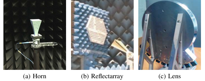
Fig. 11. Pictures of the measured antennas: (a) horn at 10 GHz in the MVG Starlab, (b) the reflectarray and (c) the Luneberg lens both measured at 12 GHz in the former CACENDRA anechoic chamber at IETR.
