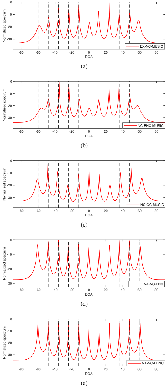
Fig. 4: Spectrum of the proposed NA-NC-BNC and NA-NC-EBNC methods, EX-NC-MUSIC method, NC-BNC-MUSIC method and NC-GC-MUSIC method, where N_1 = 3 , N_2 = 4 , \alpha = 1.5 , T = 1000 , GSNR = 10 dB, MC = 1. (a) EX-NC-MUSIC method; (b) NC-BNC-MUSIC method; (c) NC-GC-MUSIC method; (d) NA-NC-BNC method; (e) NA-NC-EBNC method.
