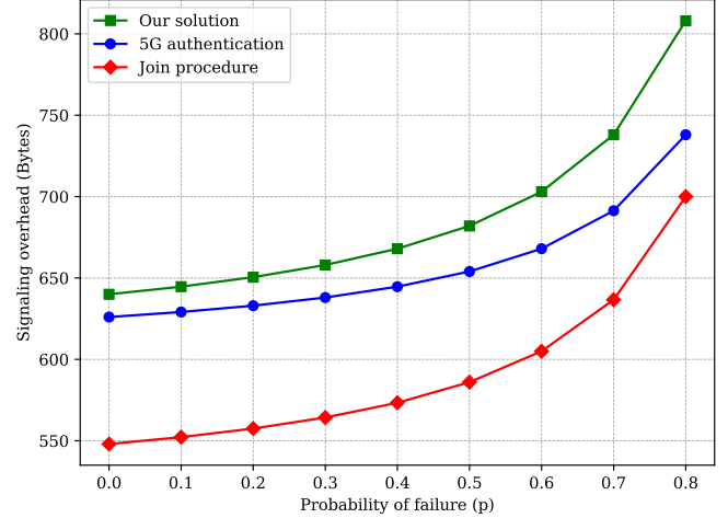
Fig. 11. Signaling overhead of access procedures in function of the probability of failure.
