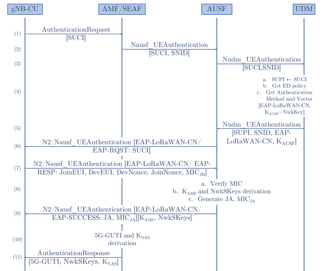
Fig. 8. The proposed primary authentication using EAP-LoRaWAN-CN.
