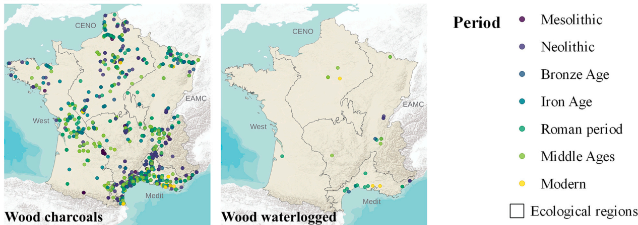
Fig. 1. Distribution of the sites included in the database according to the type of macroremains (A, Seeds and fruits; B, Wood remains) and preservation (Uncharred = waterlogged+desiccated). The color of the symbols corresponds to broad chrono-cultural periods. The French continental territory is divided into 4 broad ecological regions: Center-North (CENO), East-Massif Central (EAMC), Mediterranean (MEDIT) and West (WEST). All sites assembled in the database are represented, whether Vitis was recorded or not.
