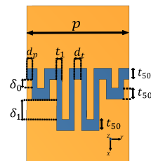
Fig. 2: Unit cell operating in spatial harmonic of n = -2 .
