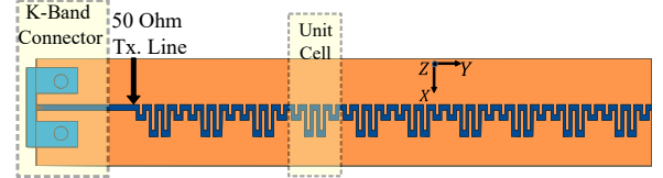
Fig. 1: Proposed LWA with 10 unit cells.
