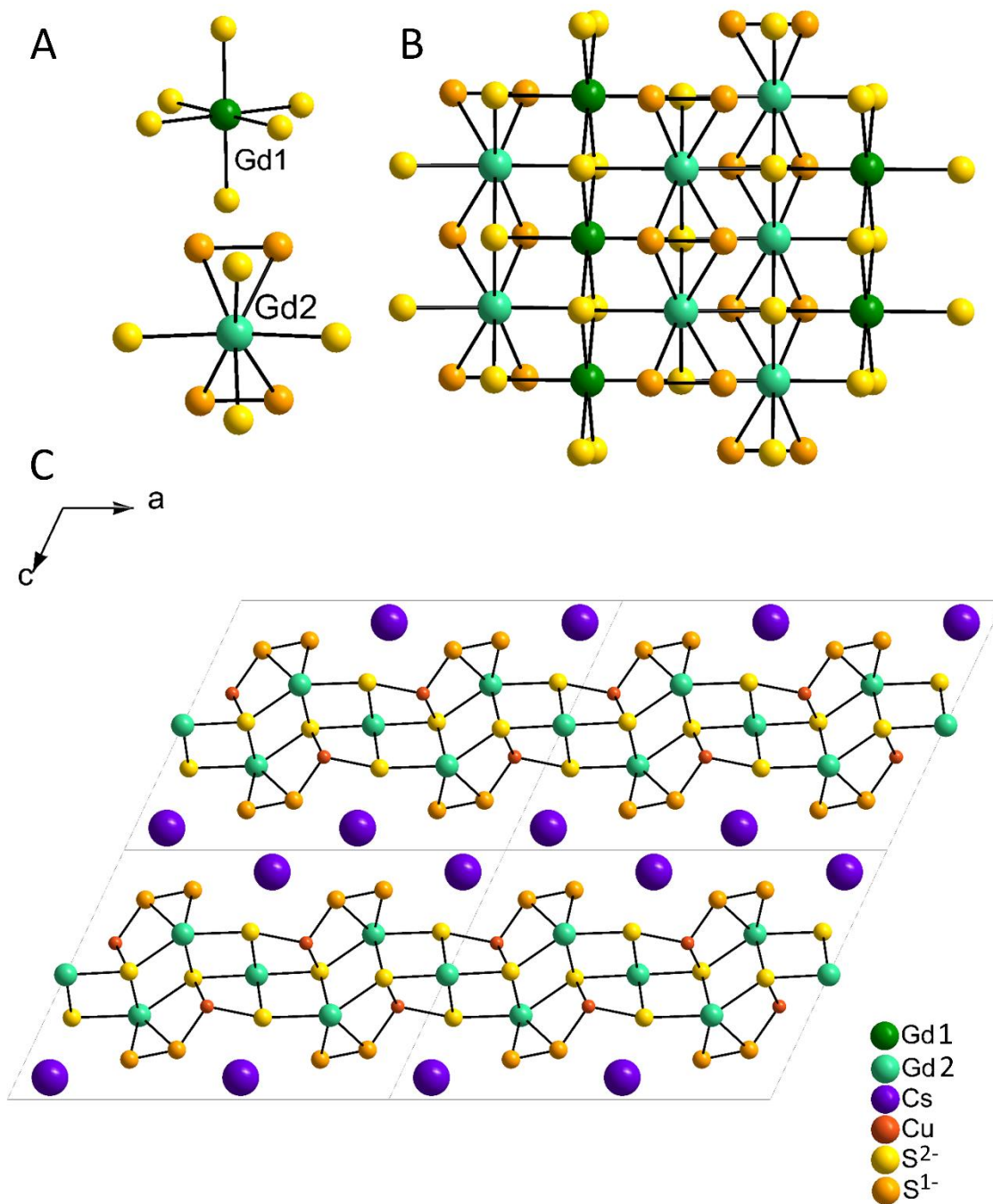
Figure 1. Crystallographic environment of \text{Ln}^{3+} cations (A), \{\text{Ln}_2\text{S}_4(\text{S}_2)_2\} \cdot \{\text{Ln}_2\text{S}_4(\text{S}_2)_2\} \cdot \{\text{LnS}_6\} part of anionic layer (B) and crystal structure of \text{Cs}_2\text{Ln}_3\text{CuS}_8 compounds (C).
