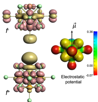
Fig. 1. Left: Fukui functions for electrophilic ( f^+ ) and nucleophilic ( f^- ) attack ( \pm 0.001 au) of \{[\text{Mo}_6\text{Cl}_8]\text{Cl}^a_5\text{Cl}^a_6\}^- . Right: Electrostatic potential (in Hartree) mapped onto the isodensity ( 0.03 \text{ e.bohr}^3 ); \vec{\mu} (6.52 Debye) by an arrow (origin \text{Mo}_6 centre).
