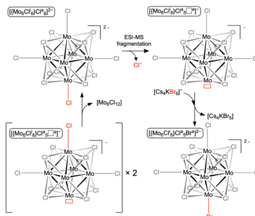
Scheme 1. Description of ESI-MS fragmentation process of [\{\text{Mo}_6\text{Cl}_8\}\text{Cl}_5\Box]^{2-} leading to [\{\text{Mo}_6\text{Cl}_8\}\text{Cl}_5\Box]^{2-} ; Reactivity of [\{\text{Mo}_6\text{Cl}_8\}\text{Cl}_5\Box]^{2-} with [\text{Cs}_4\text{KBr}_6]^- ; [\{\text{Mo}_6\text{Cl}_8\}\text{Cl}_5\Box]^{2-} self-reactivity.
