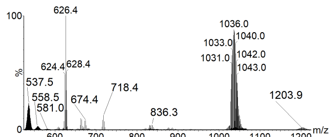
Fig. 4. Negative ESI-MS-MS spectrum of the [Mo_6Cl_{13}]^- and [Cs_4KBr_6]^- ions selected around m/z 1036 (see ESI† for more details).
