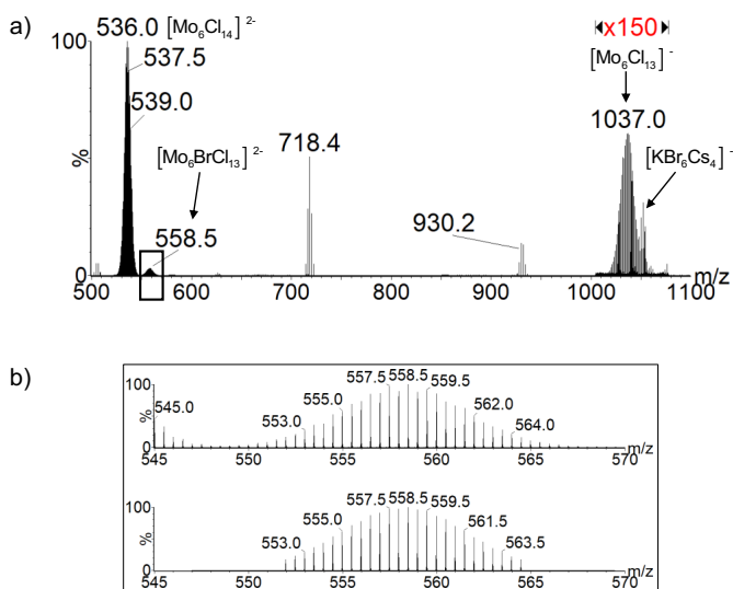
Fig. 3. a) Negative ESI-MS full-scan MS spectrum of a solution of Cs_2\{[Mo_6Cl_8]Cl^a_5\} and cesium bromide. A signal magnification of 150 times was done in the m/z 970–1070 range. The main signals at m/z 930.2 and 718.4 correspond to the [Br_3Cs_4]^- and [Br_4Cs_3]^- , respectively. b) Experimental (top) and the theoretical (bottom) isotopic patterns of the [Mo_6Cl_{13}Br]^{2-} ion ( m/z 545–575).
