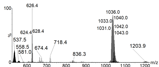
Fig. 4. Negative ESI-MS-MS spectrum of the [\text{Mo}_6\text{Cl}_{13}]^{2-} and [\text{Cs}_4\text{KBr}_6]^- ions selected around m/z 1036 (see ESI † for more details).
