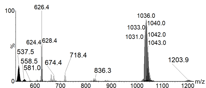
Fig. 4. Negative ESI-MS-MS spectrum of the [Mo_6Cl_{13}]^- and [Cs_4KBr_6]^- ions selected around m/z 1036 (see ESI† for more details).
