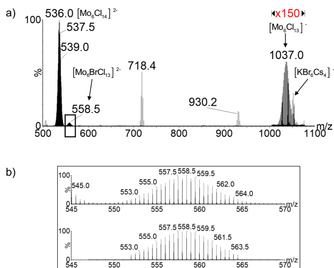
Fig. 3. a) Negative ESI-MS full-scan MS spectrum of a solution of \text{Cs}_2\{[\text{Mo}_6\text{Cl}_8]\text{Cl}^a_5\} and cesium bromide. A signal magnification of 150 times was done in the m/z 970-1070 range. The main signals at m/z 930.2 and 718.4 correspond to the [\text{Br}_7\text{Cs}_4]^- and [\text{Br}_4\text{Cs}_3]^- , respectively. b) Experimental (top) and the theoretical (bottom) isotopic patterns of the [\text{Mo}_6\text{Cl}_{13}\text{Br}]^{2-} ion ( m/z 545-575).
