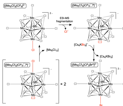
Scheme 1. Description of ESI-MS fragmentation process of [\{\text{Mo}_6\text{Cl}_8\}\text{Cl}_6]^{2-} leading to [\{\text{Mo}_6\text{Cl}_8\}\text{Cl}_5\Box]^- ; Reactivity of [\{\text{Mo}_6\text{Cl}_8\}\text{Cl}_5\Box]^- with [\text{Cs}_4\text{KBr}_6]^- ; [\{\text{Mo}_6\text{Cl}_8\}\text{Cl}_5\Box]^- self-reactivity.
