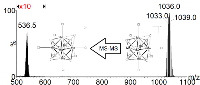
Fig. 2. Negative ESI-MS-MS spectrum of the [\text{Mo}_6\text{Cl}_{13}]^- ion selected in a mass range encompassing an experimental isotopic pattern centered at m/z 1036. Signal magnification of 10 times in m/z 500-800.
