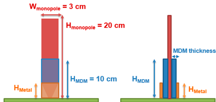
Figure 9. Final antenna topology.
