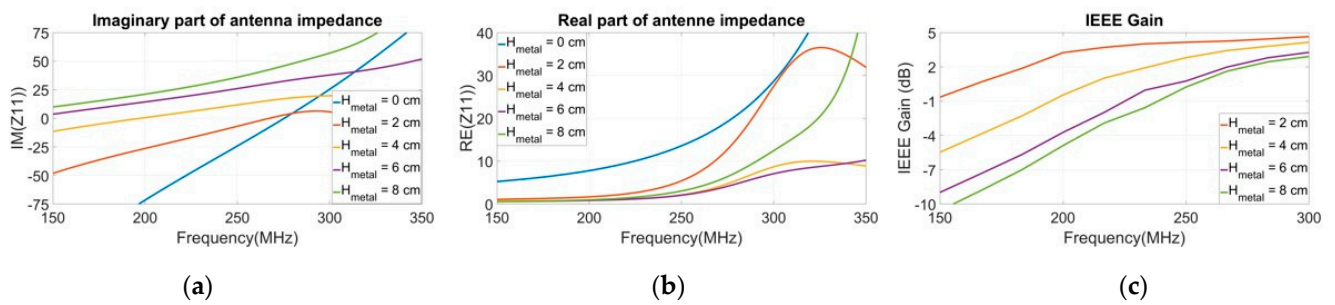
Figure 10. Effect of various metallic plates' height on the antenna: (a) imaginary part of the impedance, (b) real part of the impedance, (c) IEEE gain.
