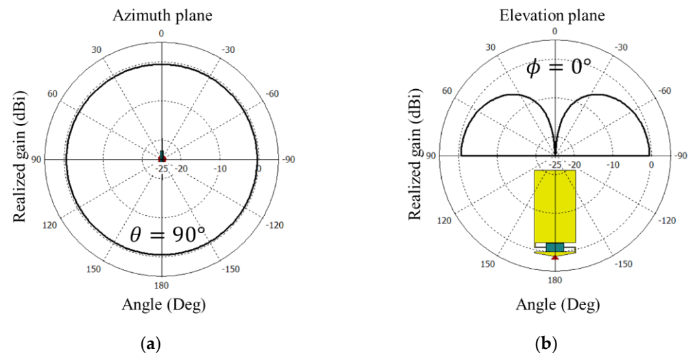
Figure 17. Simulated radiation pattern of the miniaturized and matched antenna A5 at the frequency 130 MHz. (a) in azimuth plane (b) in elevation plane.
