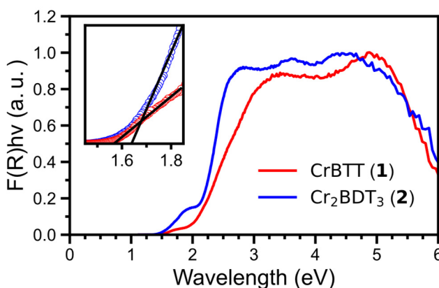
Figure 6. Normalized diffuse reflectance spectra for CrBTT ( 1 , red) and Cr 2 BDT 3 ( 2 , blue) (Inset) Corresponding Tauc plot near the band edge with extrapolation of the linear region as black lines. Experimental bandgaps via Tauc fitting: 1 = 1.57 eV, 2 = 1.64 eV (Fig S12).
