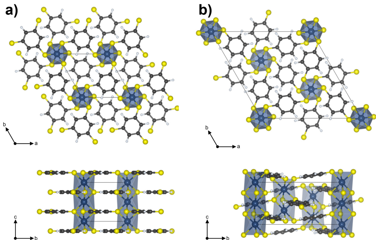
Figure 2. The refined CP structure unit cells as viewed along the c and a axes with (CrS 3 ) n chains depicted as metal-centred polyhedra. (a) The structure of CrBTT ( 1 ), a = 7.821(3) \text{ \AA} , c = 6.064(1) \text{ \AA} . (b) The structure of Cr 2 BDT 3 ( 2 ), a = 15.382(1) \text{ \AA} , c = 6.4693(4) \text{ \AA} , depicted here in the trigonal rather than rhombohedral unit cell for comparison.
