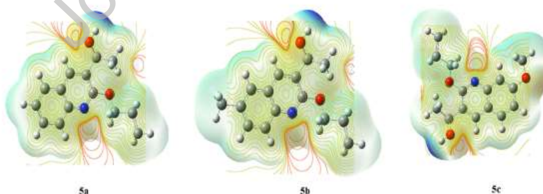
Fig.3. The MEP surfaces of compounds ( 5a-c ).
