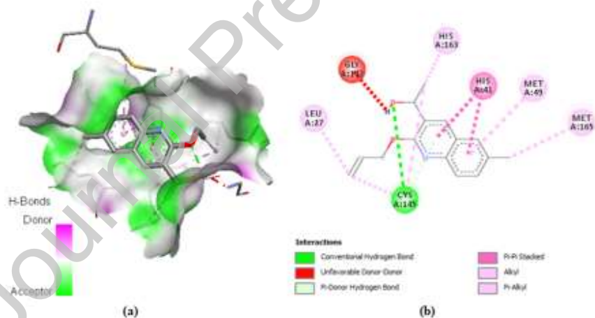
Fig. 6. (a) 3D and (b) 2D molecular docking results of the compound (5b) + 6LU7.
