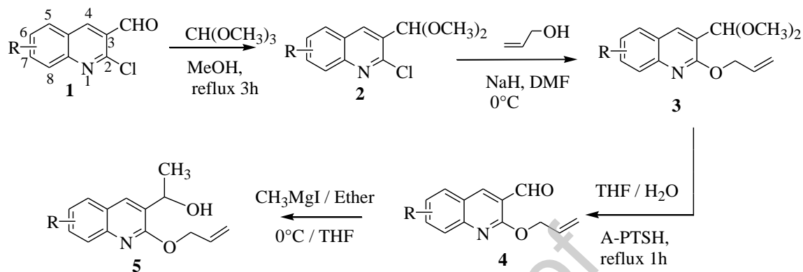
Scheme 1. Synthesis of compounds (5a-c).
