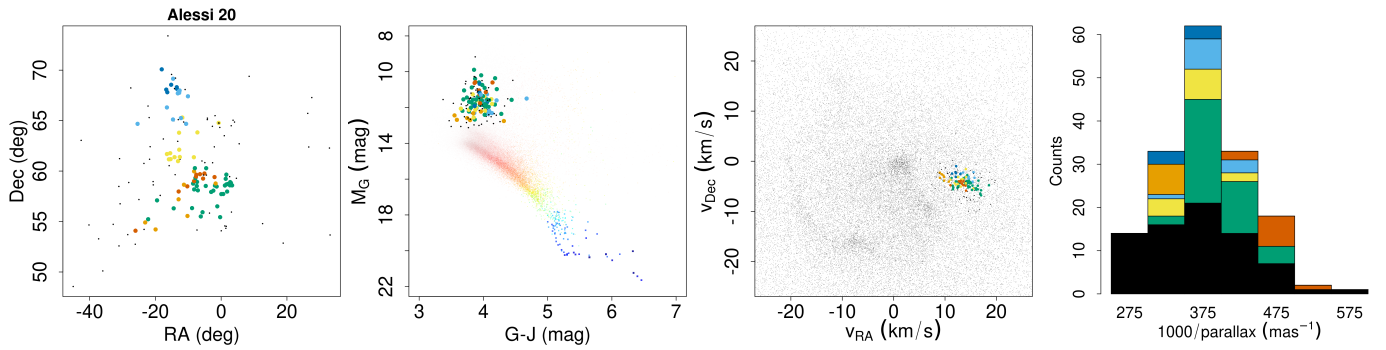
Fig. C.14: Same as Fig. C.1 but for the region near Alessi 20.
