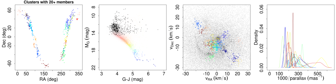
Fig. C.15: Same as Fig. C.1 but for the rest of clusters with more than 20 members. We use different colours for the various clusters, except for the CAMD, to avoid confusion with the colour code that reflects T_{\text{eff}} along the main sequence.
