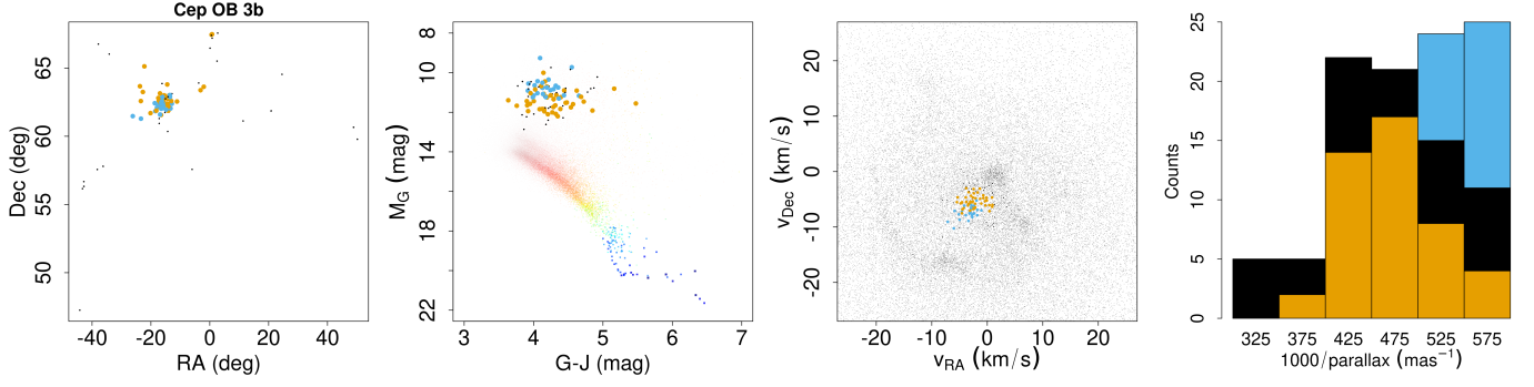
Fig. C.7: Same as Fig. C.1 but for Cep OB 3b.
