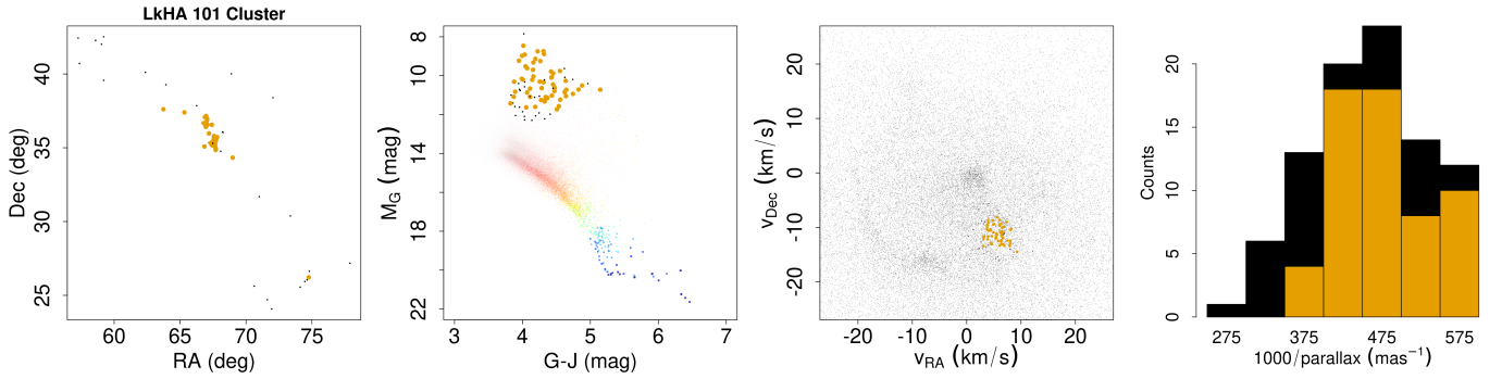
Fig. C.8: Same as Fig. C.1 but for the LkHA 101 Cluster.
