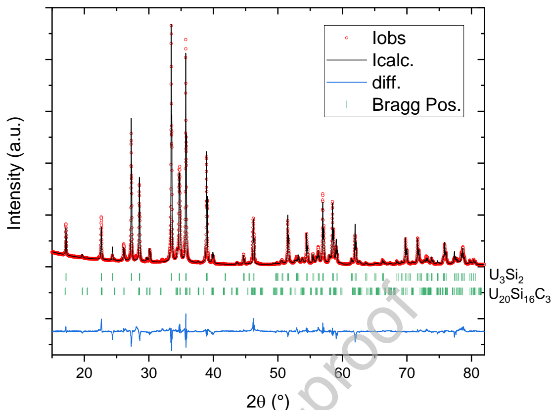
Figure 3: XRD pattern refined using the Rietveld method for batch C of atomized \text{U}_3\text{Si}_2 powder. The experimental data are plotted in red, the calculated ones in black and their difference is drawn in blue. The vertical green ticks indicate the Bragg peaks positions for \text{U}_3\text{Si}_2 and \text{U}_{20}\text{Si}_{16}\text{C}_3 -like phases. Agreement factors: R_{\text{Bragg}}(\text{U}_3\text{Si}_2) = 9.8\% ; R_{\text{Bragg}}(\text{U}_{20}\text{Si}_{16}\text{C}_3) = 19.6\% ; \chi^2 = 24.0 .
