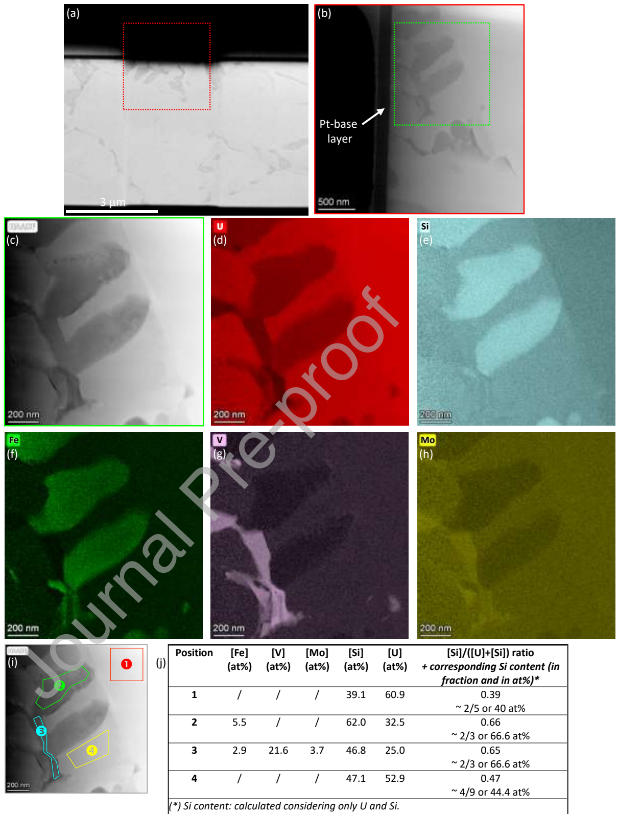
Figure 11: STEM + EDS analysis of a FIB lamella taken from a polished section of a particle from batch C of atomized U_3Si_2 powder - (a) (b) general views of the lamella respectively taken by SEM (BSE mode) and STEM (HAADF mode), (c) STEM-HAADF image of the area analysed by EDS, (d) (e) (f) (g) (h) X-ray maps for U (in red), Si (in light blue), Fe (in green), V (in light purple) and Mo (in yellow), (i) location of parts of the map for which corresponding quantitative results are given in (j).
