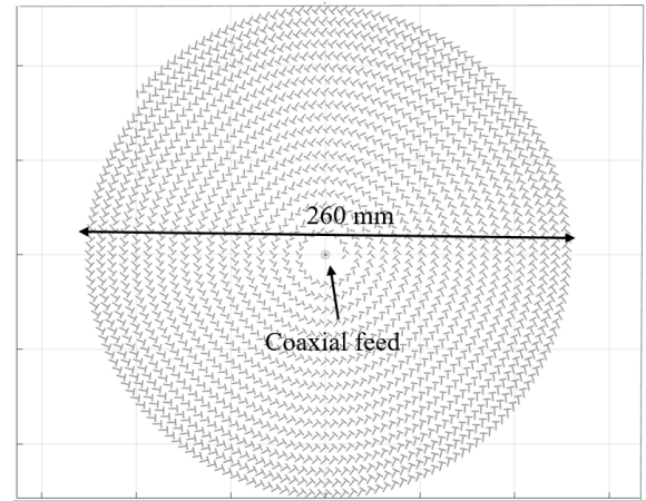
Fig. 5. The layout of the optimized standard RLSEA
