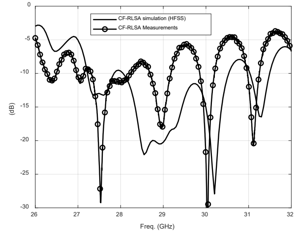
Fig. 17. Measured and simulated reflection coefficient of CF-RLSA
