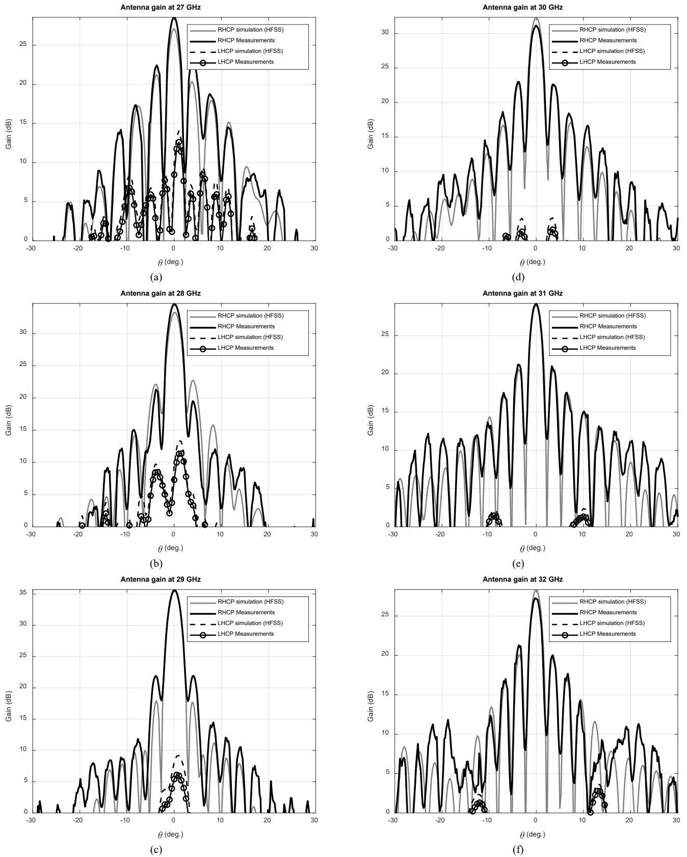
Fig. 13. Measured and simulated gain patterns ( \phi = 0^\circ ) at (a) 27, (b) 28, (c) 29, (d) 30, (e) 31 and (f) 32 GHz.
