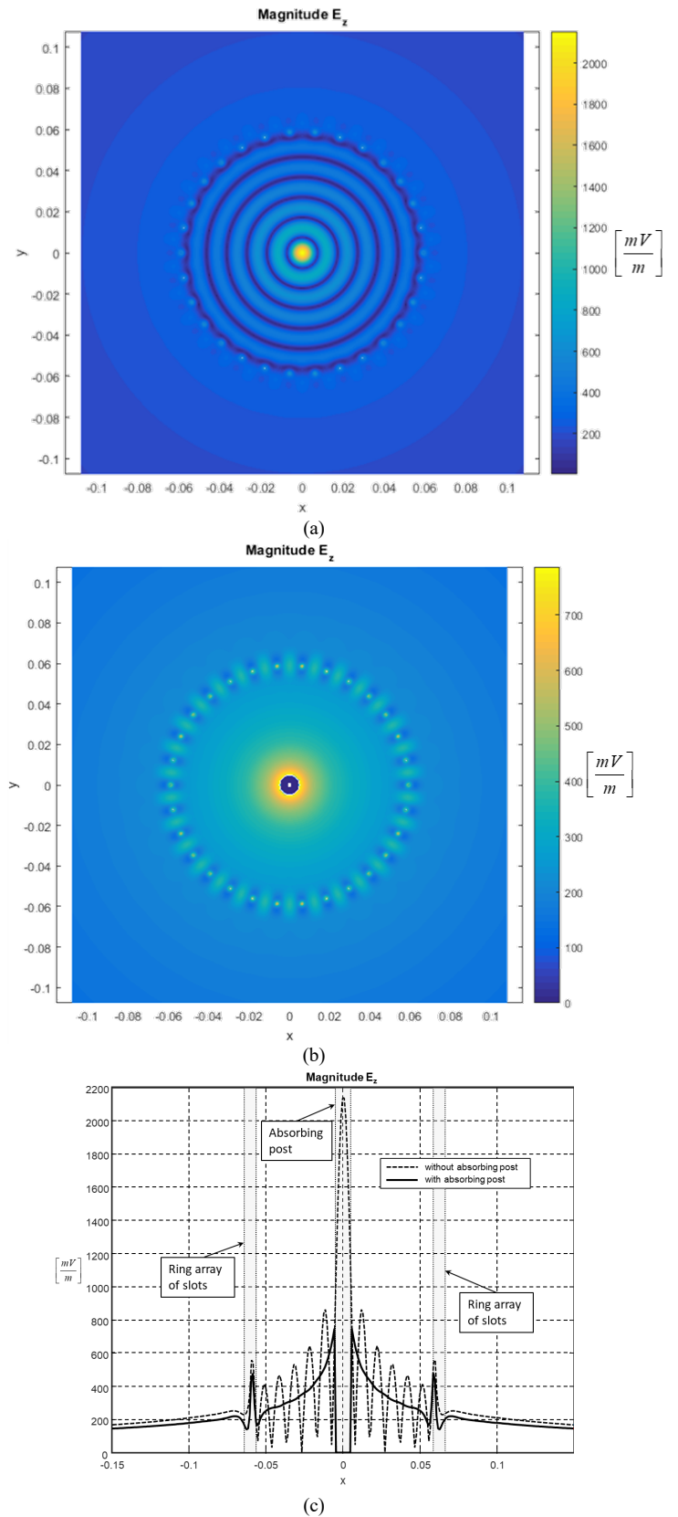
Fig. 7. Electric field launched by the feeder in the upper PPW (absence of radiating slots). (a) Stationary wave presence in the internal area. (b) Effect of the introduction of the absorbing central post. (c) Comparison of the radiation patterns in the horizontal cut-plane with and without the central absorbing pin.
