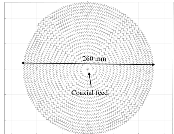
Fig. 5. The layout of the optimized standard RLSA
