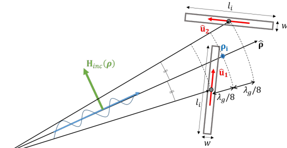
Fig. 4. Geometry of the i^{\text{th}} slot pair, radiating a right-handed circular polarized field when illuminated by an outward propagating incident field \mathbf{H}_{\text{inc}}(\rho) .
