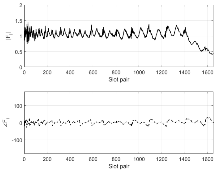
Fig. 9. The amplitude and phase of the fitness function at the end of the optimization procedure
