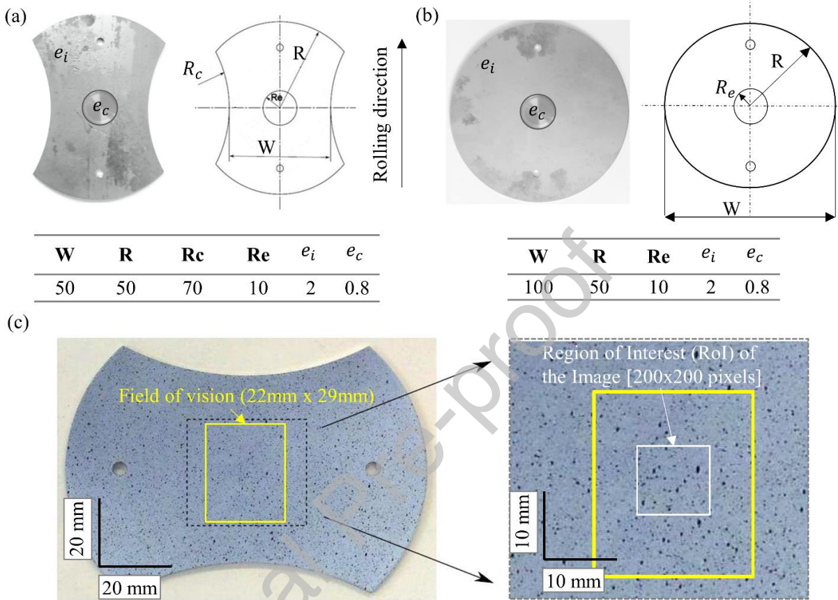
Fig. 4 Marciniak specimens' forms and dimensions (a) specimen dimensions in the plane expansion condition: R being the radius of the tested specimen, R_c being the radius of the outer curves and W being the width of the specimen, e_i being the initial specimen thickness and e_c being the thickness of the central zone (b) specimen dimensions in the biaxial expansion condition [56]: R being the radius of the tested specimen and R_e being the radius of the central zone where thickness reduction is applied for strain localization, e_i being the initial specimen thickness and e_c being the thickness of the central zone (c) Black and white speckled sample before Marciniak testing [56]. The yellow rectangle corresponds to the field of vision of the cameras and the white one corresponds to the region of interest (ROI). To note that all dimensions are given in mm.
