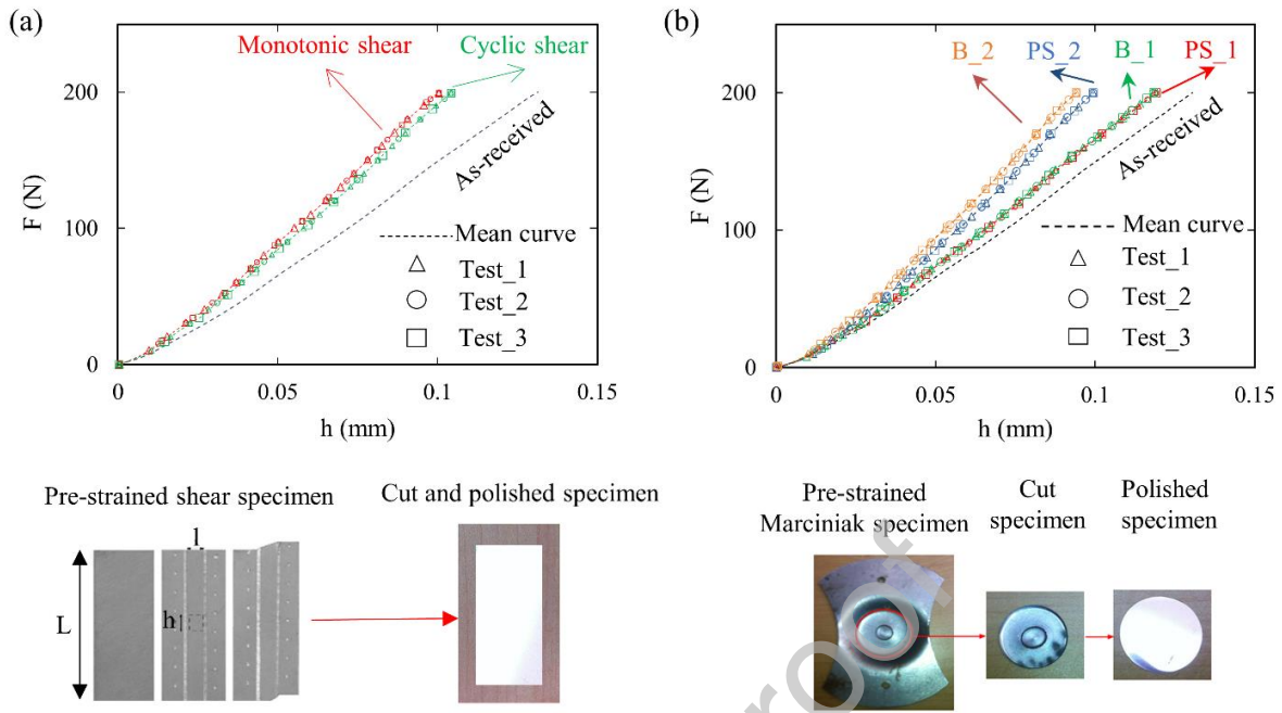
Fig. 7 (a) F (N) – h (mm) indentation curves before and after pre-straining by monotonic and cyclic shearing and corresponding specimens' preparation. Results are in agreement with what was obtained in Fig. 3-d where for approximately the same pre-strain level, monotonic shearing led to a cumulative stress value higher than the one obtained in the case of cyclic shearing (b) F (N) – h (mm) indentation curves obtained for as-received and Marciniak pre-strained specimens and corresponding specimens' preparation. Results are in agreement with the values presented in Table 3 and Fig. 6 where for PS_1 and B_1 (small displacements), the corresponding indentation curves show less resistance than the ones obtained for PS_2 and B_2 (large displacements)
