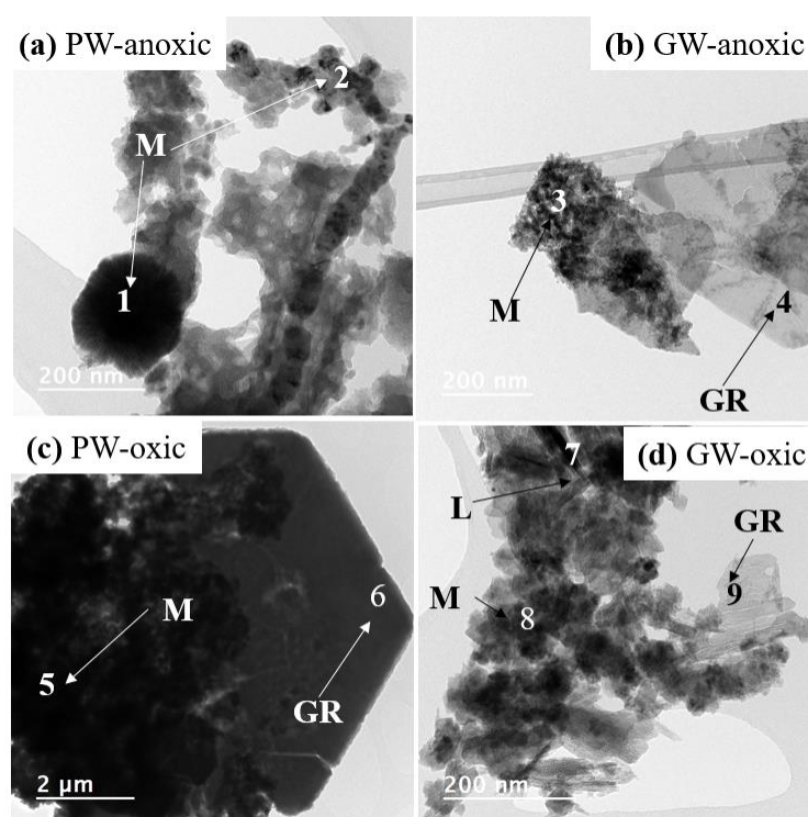
390 Figure 5. Transmission electron microscopy images of NZVI aging products at 60 days 391 under different conditions: (a) PW- anoxic system, (b) GW-anoxic system, (c) PW-oxic 392 system, and (d) GW-oxic system. Note: M: magnetite/maghemite; GR: green rust; L: 393 lepidocrocite; GW: groundwater; PW: pure water. (Electron diffraction patterns of the
