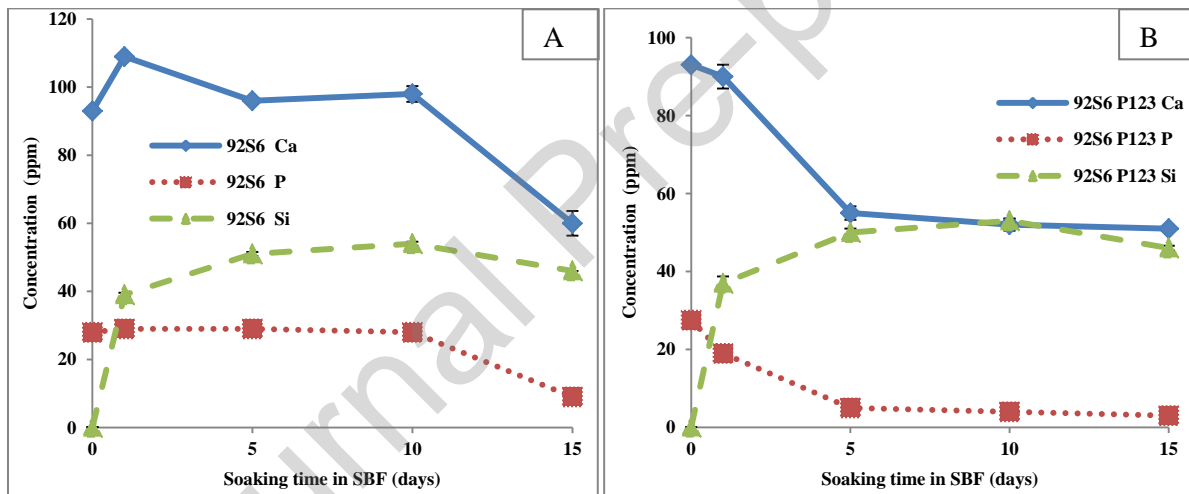
Figure 4. Evolution of (Ca), (P) and (Si) concentrations in SBF versus time soaking. A: 92S6, B: 92S6 P123.
