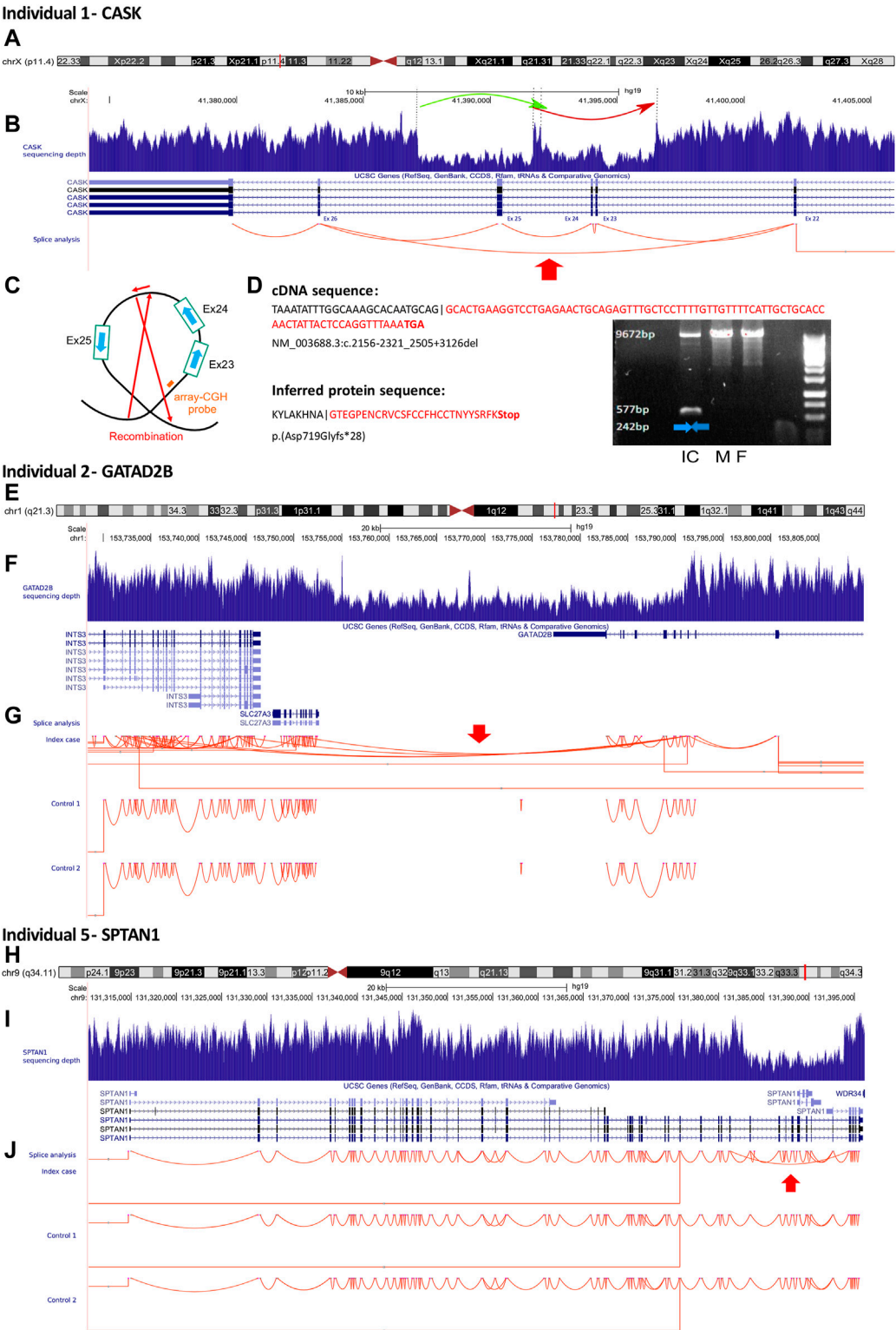
FIGURE 3 Illustration of individuals 1—CASK, 2—GATAD2B, and 5—SPTAN1. (A) Ideogram showing chromosome X and CASK localization. Under the ideogram, the green and red arrows represent the deletion-inversion of 9.4 kb in Xp11.4. (B) UCSC genome browser snapshot with visualization of CASK sequencing depth and CASK splice analysis. CASK sequencing depth demonstrates an intragenic deletion encompassing exons 23 through 25. The red arrow in the splicing analysis demonstrates the presence of a heterozygous transcript lacking exons 23 through 25. (C) Graphic (Continued)
