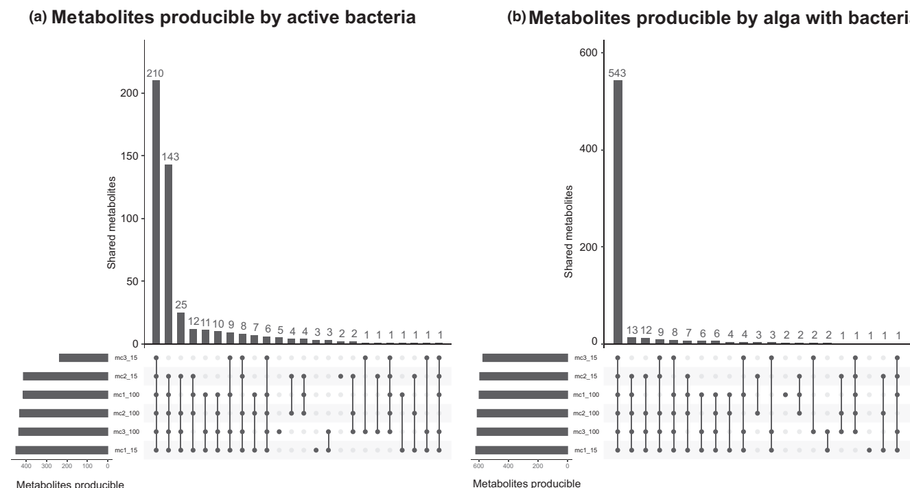
FIGURE 7 Upset plot of (a) metabolites predicted to be producible by the active bacterial communities in the different conditions, and (b) metabolites predicted to be newly producible by the algal host if given access to the metabolites producible by the bacteria. The bars represent the number of metabolites shared between the different communities and conditions. Most metabolites are producible in all communities, but MC3–15% has the lowest number of producible metabolites. A detailed list of metabolites is available in Table S11
