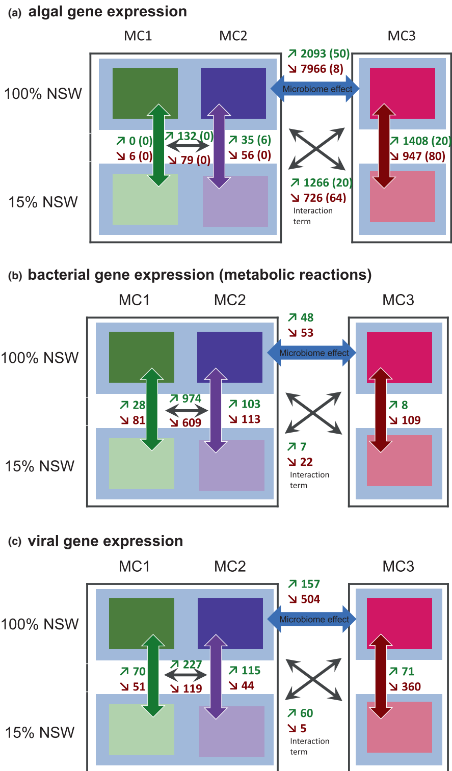
FIGURE 4 (a) Differentially expressed algal genes. The figure shows the number of differentially expressed algal genes with each of the microbial communities in 15% NSW compared to 100% NSW (MC1, MC2, and MC3); algae with MC1+MC2 jointly compared to those with MC3 in 100% NSW (microbiome effect), the differences between algae with MC1 and MC2, and the difference in the low salinity-response of algae with MC3 compared to those with MC1+MC2 (interaction term, crossed arrows). Numbers in parentheses correspond to the number of overrepresented GO terms associated with the differentially regulated genes. (b) Similar analysis as A, but on the bacterial transcriptome; in this case, the analysis was based on differentially expressed metabolic reactions rather than genes. (c) Similar analysis as (a) and (b), but concerning viral sequences. Samples with MC3 exhibited the strongest host response, while the bacterial responses were equally pronounced for all three MCs
