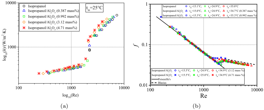
Fig. 7 Results of the experiments in transition region presented by Nikulin et al. [18], for a) heat transfer, b) friction factor. Reprinted with permission from Elsevier with the license number 5025290624013.
