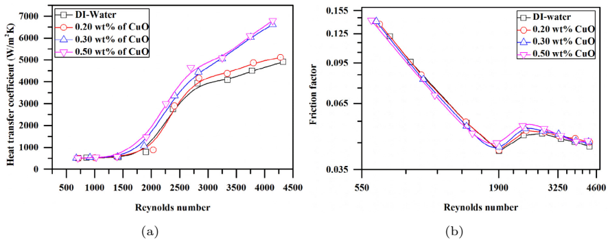
Fig. 10 Results of the experiments in transition region presented by Khairul et al. [40], a) heat transfer, b) friction factor. Reprinted with permission from Elsevier with the license number 5025291205236.
