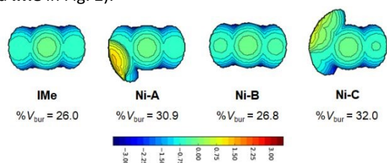
Fig. 2 Steric maps and %V bur values of NHCs IMe , Ni-A , Ni-B and Ni-C calculated with SambVca 2.1 with the following standard inputs: Bondi radii 1.17 Å, Rh II -C NHC 2.00 Å, r sphere = 3.50 Å, mesh spacing 0.10 Å, H atoms excluded, see ref. 11.
