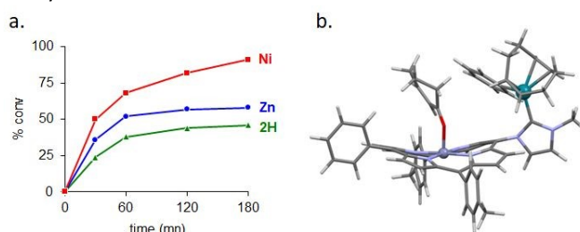
Fig. 4 a. Time-dependent reaction profiles of the conjugate addition of phenylboronic acid to cyclohexen-2-one catalysed by M 1 -C-Rh(cod)Cl (M 1 = Ni in red, Zn in blue and 2H in green) in toluene at 100 °C. b. PM3-minimized molecular modelling of a plausible transition state of Ni-C-Rh(cod)Cl with phenyl and cyclohexen-2-one bonded to Rh(I) and Ni(II), respectively.
