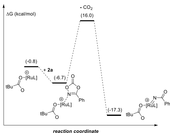
Fig. 3 Reaction profile of the extrusion of CO 2 with the coordination of dioxazolone in 10' . Relative Gibbs energies relative to I (in kcal/mol). L = p -cymene.
