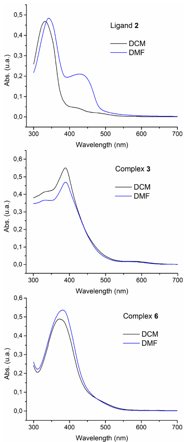
Figure 4. UV/vis spectra of Schiff base proligand 2 (top), complexes 3 (middle) and 6 (bottom) recorded in DCM (black line) and DMF (blue line) solutions.
