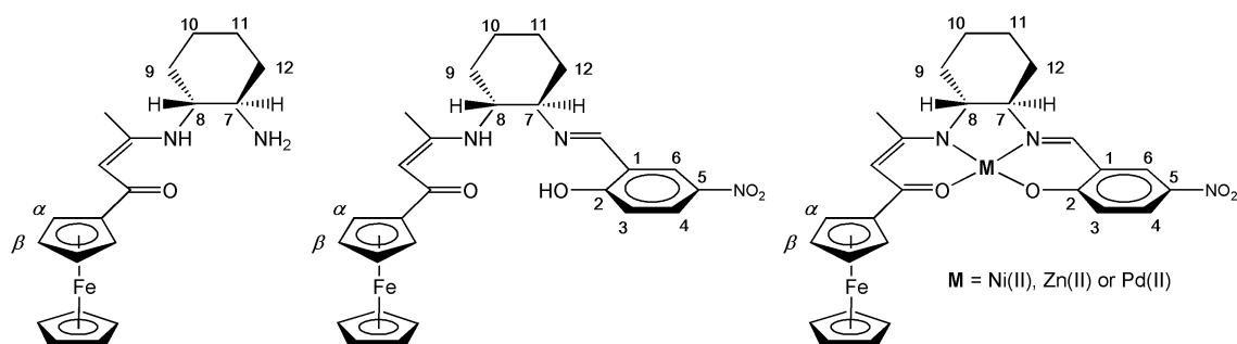
Figure 7. Labeling scheme used for NMR assignments.
