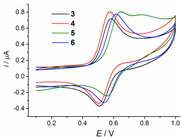
Figure 3. Cyclic voltammograms of complexes 3-6 recorded at a glassy carbon working electrode in DMF containing 0.1 M [ n -Bu 4 N][PF 6 ] at T = 298 K with a sweep rate \nu = 0.1 V s -1 , reference electrode Ag/AgCl. The second redox event observed in the Zn II complex 5 could be attributed to an adsorption process.
