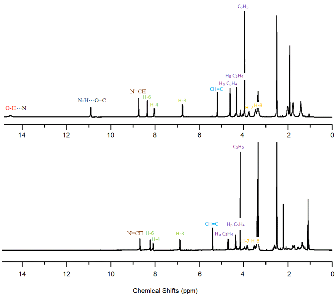
Figure 1. 1 H NMR spectra (400 MHz) of metalloligand 2 (top) and of its related Pd(II) complex 6 (bottom), recorded in [D 6 ]DMSO at 298 K.
