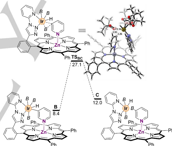
Figure 4. Probing the iridium-mediated meta -carbon-borylation step in a pyridine substrate. B = (pinacol)boron. Relative Gibbs free energies in kcal/mol, selected distances in Å.
