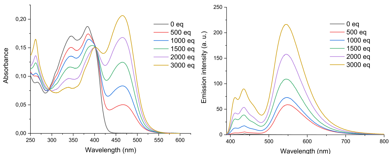
Figure 6. Changes in the absorption (left) and emission (right, \lambda_{\text{exc}} = 384 nm) spectra of a \text{CH}_2\text{Cl}_2 solution of 4a ( c = 4.12 \times 10^{-6} M) upon addition of TFA.
