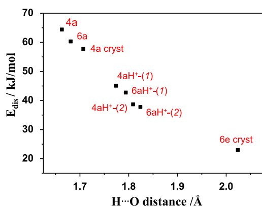
Figure 12. Dependence of the dissociation energy ( E_{\text{dis}} ) vs H...O distance.
