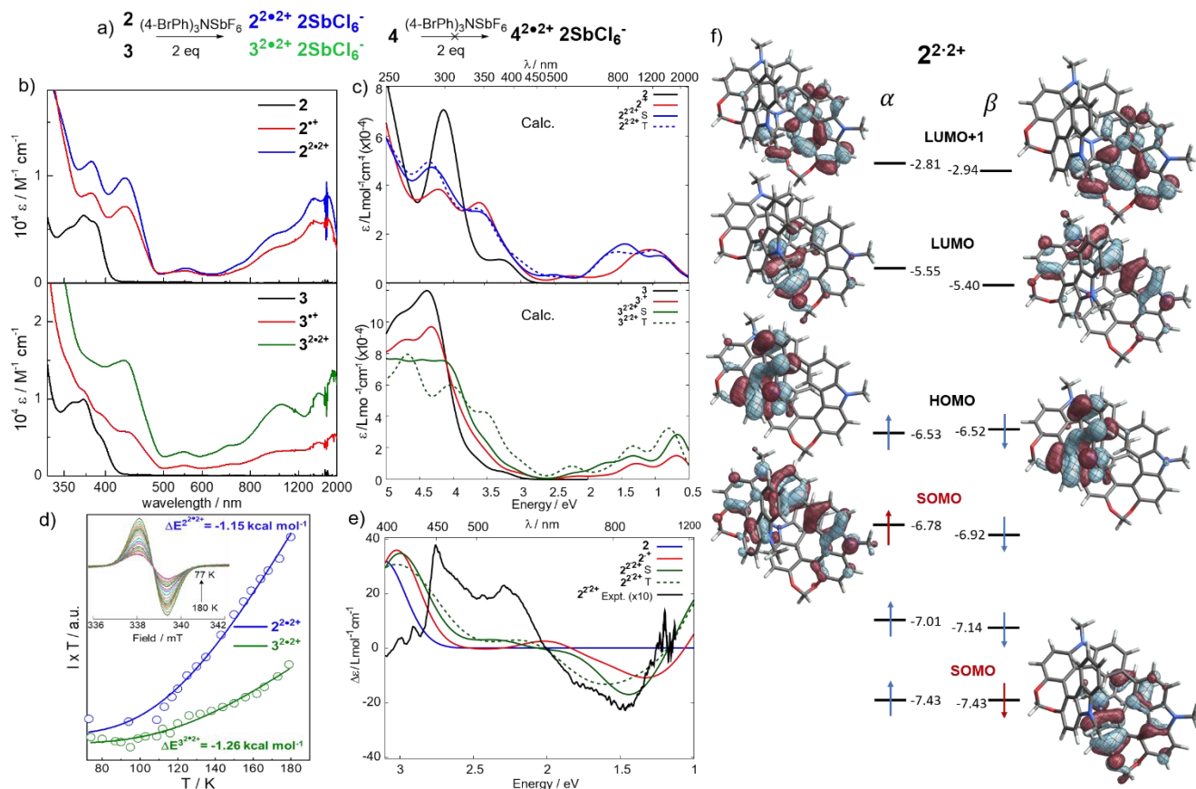
Figure 5. a) Synthetic route to persistent radicals 2^{2\cdot 2+} \mathbf{2SbCl}_6^- , 3^{2\cdot 2+} \mathbf{2SbCl}_6^- , and 4^{2\cdot 2+} \mathbf{2SbCl}_6^- . b) UV-vis-NIR absorption spectra of: 2 (black), 2^{2+} \mathbf{SbCl}_6^- (red) and 2^{2\cdot 2+} \mathbf{2SbCl}_6^- (blue) (top), and 3 (black), 3^{2+} \mathbf{SbCl}_6^- (red) and 3^{2\cdot 2+} \mathbf{2SbCl}_6^- (green) (bottom) in dichloromethane at 298 K; c) Calculated UV-vis-NIR absorption spectra of top: 2 (black), 2^{2+} \mathbf{SbCl}_6^- (red) (top), and 2^{2\cdot 2+} \mathbf{2SbCl}_6^- (blue) and bottom: 3 (black), 3^{2+} \mathbf{SbCl}_6^- (red) and 3^{2\cdot 2+} \mathbf{2SbCl}_6^- (green) in dichloromethane. d) I \times T vs. T plots of frozen solution of diradicals 2^{2\cdot 2+} \mathbf{2SbCl}_6^- (blue) and 3^{2\cdot 2+} \mathbf{2SbCl}_6^- (green) in dichloromethane fitted using Bleaney-Bowers model with an estimated average \Delta E_{ST} values obtained from two measurements. e) Experimental vis-NIR ECD spectrum of 2^{2\cdot 2+} \mathbf{2SbCl}_6^- (black) and calculated vis-NIR ECD spectra of (+)- 2 (blue), (+)- 2^{2+} (red) and (+)- 2^{2\cdot 2+} (green) for both singlet (solid line) and triplet (dashed line) spin multiplicity; f) Top: Isosurfaces ( \pm 0.030 a.u.) of frontier molecular orbitals computed for diradicals 2^{2\cdot 2+} .
