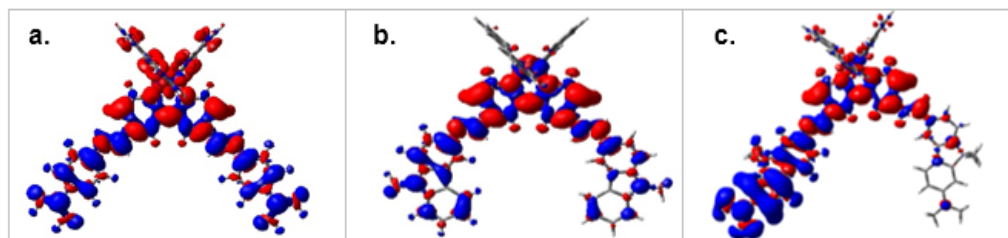
Figure 5. (a–c) PBE0-GD3BJ/LANL2DZP density differences plots ( D\rho(r) = \rho^{S1}(r) - \rho^{S0}(r) ) of [\text{RuL}(\text{bpy})_2]^{2+} complexes, (a) L = L^T , (b) L = L^C , and (c) L = L^F between S_1 and S_0 states (red = increase, blue = decrease of electron density; iso-value 0.03 au).
