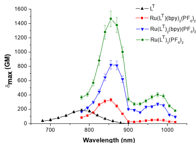
Figure 2. TPA spectra of L^T and [Ru(L^T)_{3-n}(bpy)_n]^{2+} ( n = 0-2 ) complexes; THF, c = 1.0 \times 10^{-5} \text{ mol.L}^{-1} .
