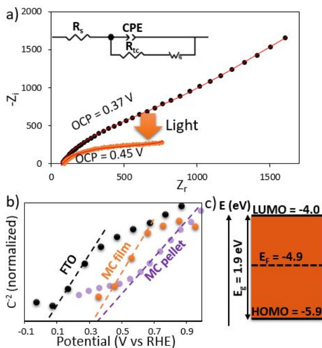
Figure 5. Transient (photo)-electrochemical measurements. a) Nyquist diagrams of electrochemical circuit in dark and under illumination at open circuit potential and the equivalent circuit used to fit them. b) Mott-Schottky plots for the MC film deposited on FTO, the FTO substrate and the \text{Cs}_2[\{\text{Mo}_6\text{I}_8\}\text{I}_6] dense pellet depicted versus RHE by using the formulae V_{fb}(\text{RHE}) = V_{fb}(\text{Ag}/\text{AgCl}) + 0.059 \text{ pH} + V_{\text{Ag}/\text{AgCl}}(\text{RHE}) 23 c) Energy levels (absolute scale with
