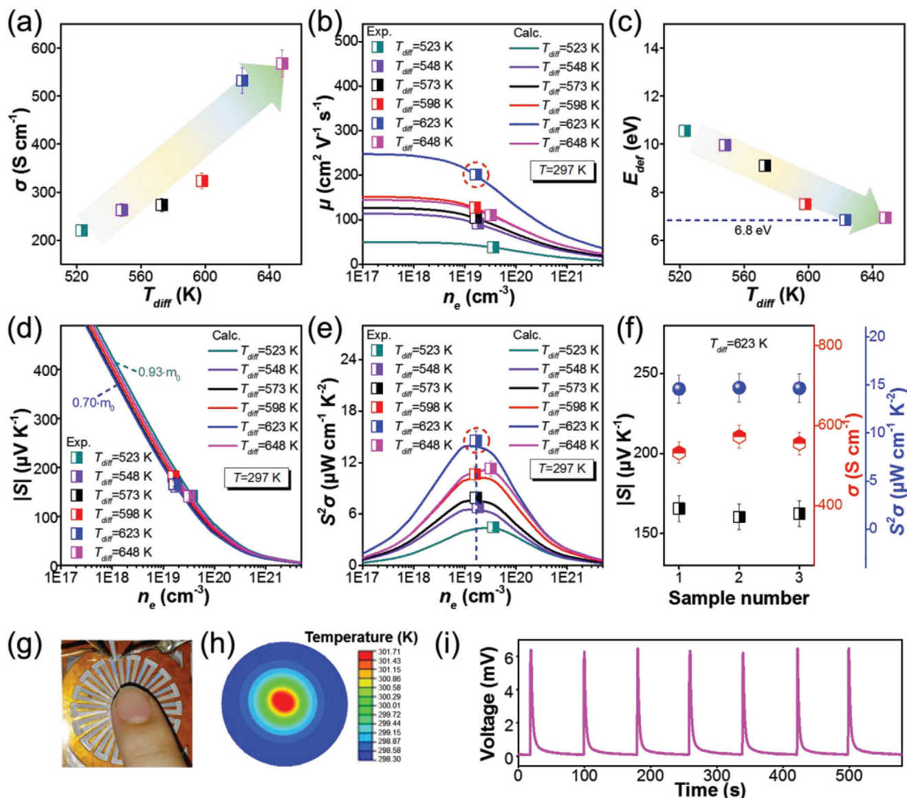
Figure 5. a) Measured \sigma of as-prepared Bi 2 Te 3 -based flexible thin films as a function of diffusion temperature. b) Measured \mu as a function of n_e in comparison with the SPB model calculated values. c) E_{def} as a function of diffusion temperature. d) Measured |S| as a function of n_e in comparison with the SPB model calculated values. e) Measured S^2\sigma as a function of n_e in comparison with the SPB model calculated values. f) Repeatedly measured room-temperature \sigma , |S| and S^2\sigma of Bi 2 Te 3 flexible thin film prepared under the diffusion temperature of 623 K. g) Optical photo of a finger contact on thin film thermoelectric sensor with corresponding h) calculated temperature distribution and i) the output voltage signals.
