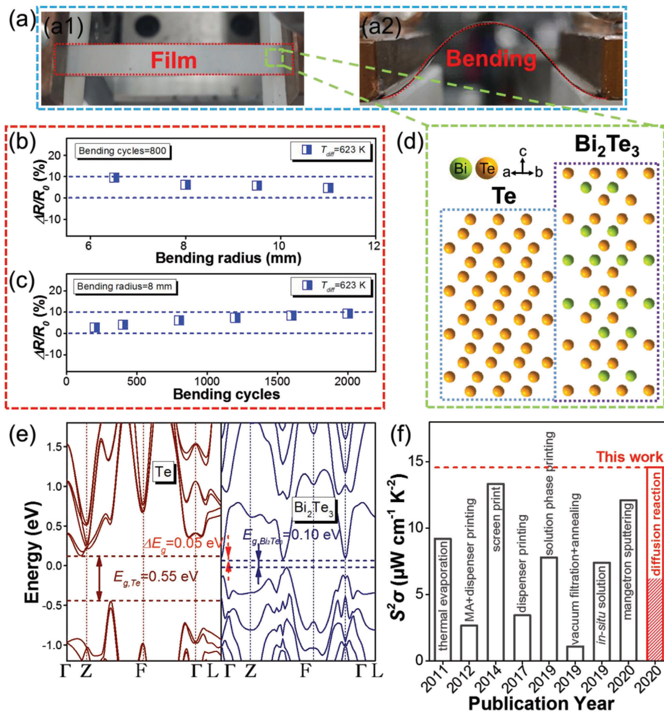
Figure 1. a) Optical images of as-prepared Bi_2Te_3 flexible thin film under (a1) flat and (a2) bending statuses, respectively. b) The \Delta R/R_0 of the Bi_2Te_3 flexible thin film prepared under the diffusion temperature of 623 K as a function of bending radius at the bending cycles of 800 times. c) The \Delta R/R_0 of the Bi_2Te_3 flexible thin film prepared under the diffusion temperature of 623 K as a function bending cycles at the bending radius of 8 mm. d) Schematic structure of Bi_2Te_3 and Te. e) DFT calculated electronic band structures of Te and Bi_2Te_3 , respectively. f) Comparison of the maximum room-temperature S^2\sigma between our Bi_2Te_3 -based flexible thin films and other state-of-art n-type Bi_2Te_3 -based flexible thin films prepared by different methods, including thermal evaporation (2011), [35] mechanically alloyed (MA) and dispenser printing (2012), [19] screen print (2014), [34] dispenser printing (2017), [32] solution phase printing (2019), [30] vacuum filtration and annealing (2019), [31] in situ solution (2019), [33] magnetron sputtering (2020), [36] and this work.
