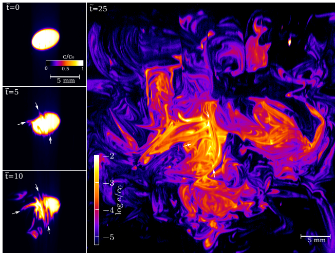
FIG. 1. Heterogeneous and anisotropic scalar signature of the push-pull echo during a push-pull experiment through random bead packings. The initially spheroidal dye blob at \bar{t} = t'\bar{u}/d = 0 diffuses preferentially along directions of high fluid deformation (indicated by arrows), leading to a highly striated dye distributions at later times. See video in [9].
