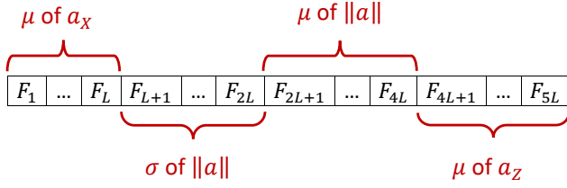
Fig. 4. The 5L extracted features using online computation.
