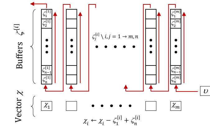
Fig. 3. The process consists of m buffers \zeta_j^{[i]} of length n . The red arrows indicate the propagation of acquired data-points. For each new read value \nu , the \zeta_j^{[i]} values are shifted by one sample, \zeta_1^{[i]} is excluded, and the elements \chi_i are updated as indicated in the figure.
