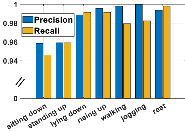
Fig. 8. The performance of MDA in terms of precision and recall for each targeted ADL using 1-vs-all strategy.
