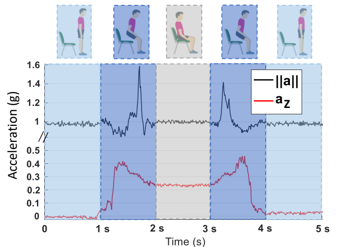
Fig. 2. The stand-to-sit and sit-to-stand (dark blue) are represented by two opposite sine waves in acceleration magnitude ||a|| . The a_Z component, directed towards the human trunk, fluctuates during these two transitions.
