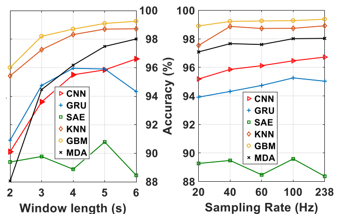
Fig. 9. The achieved accuracies (%) when (i) F_s is fixed and L is variable (left graph) and (ii) L is fixed and F_s is variable (right graph).
