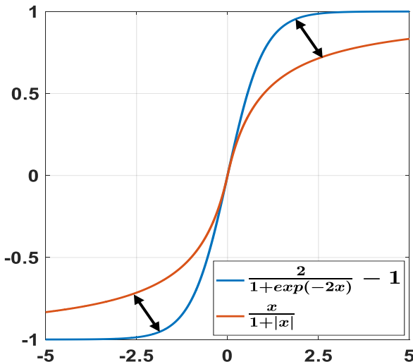
Fig. 5. Hyperbolic tangent sigmoid (blue) vs customized function (orange).
