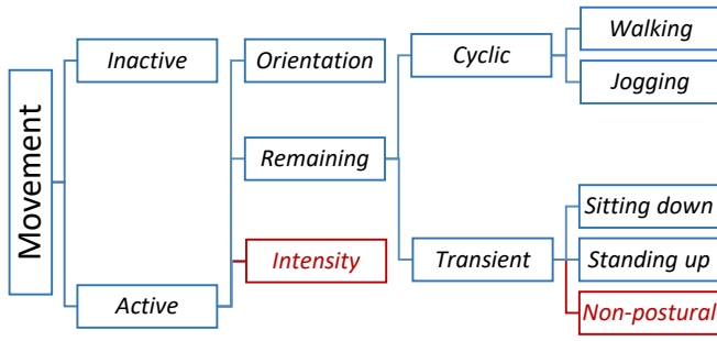
Fig. 1. The steps of the proposed HAR approach, starting from data acquisition to predict the activity (blue leaf) or exclude it (red leaf).
