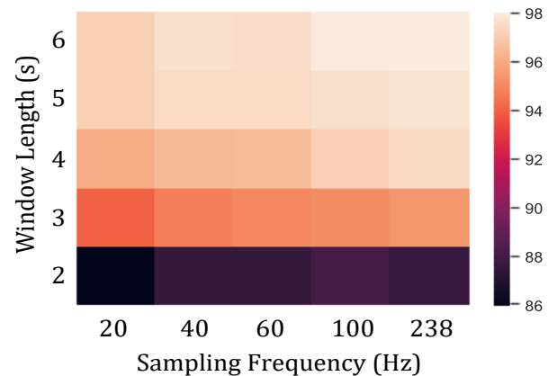
Fig. 7. The heat map consisting of the achieved accuracy (%) for each (F_s, L) pair after applying MDA.
