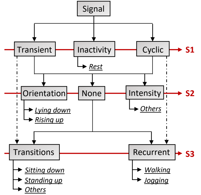
Fig. 6. The proposed multinomial decomposition algorithm, consisting of three stages S1 \rightarrow S3 , which predicts the performed ADL at a low-cost.
