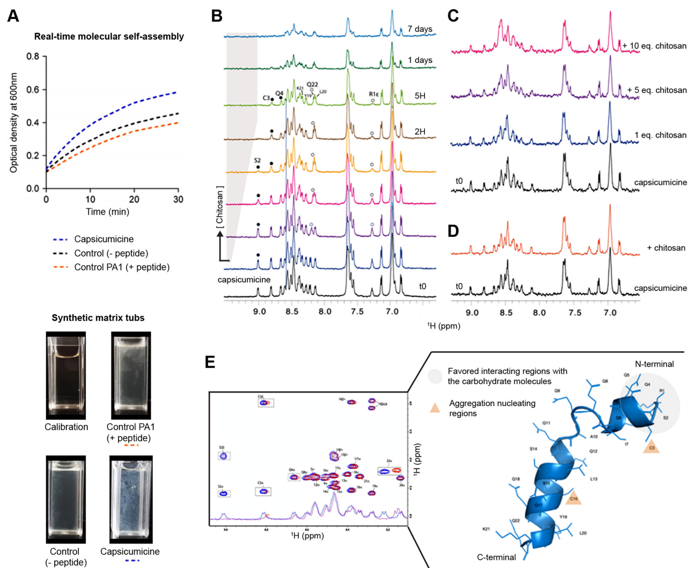
FIG 3 Molecular interactions between capsicumic acid and target-saccharides. (A) RTMSA curves of artificial staphylococcal biofilm assembly. Optical densities ( OD_{600} ) were recorded as a function of the time in the presence of capsicumic acid (blue dots) or PA1 as peptide control (orange dots) and the synthetic matrix without peptides (black dots); each reaction tub is shown under the graph. (B-D) NMR titration of capsicumic acid by chitosan at 600 MHz, 10°C. (B) From the bottom to the top: increasing concentrations of soluble chitosan [ <0.5 eq. and 8% of volume variation] were gradually added to capsicumic acid water solution. Specific line broadenings and frequency shifts are shown in the NMR spectrum for some amide protons upon titration; white bullets for terminal R1 and Q22 and black bullets for S2, C3 and Q4. (C) Assembled chitosan gradually added to soluble capsicumic acid [0.5 eq.]; an overall line broadening was observed. (D) Assembled chitosan suddenly added to soluble capsicumic acid [0.5 eq.]; the orange spectrum was recorded after few minutes of stirring. (E) Superposition of capsicumic acid 1D NMR and TOCSY spectra immediately after sample preparation (blue) and chitosan [10 eq.] addition (red) and; capsicumic acid structure predicted by Phyre2 server; according to NMR results the aggregation nucleating regions are shown as orange triangles and favored interacting region with sugar moieties is shown in gray.
