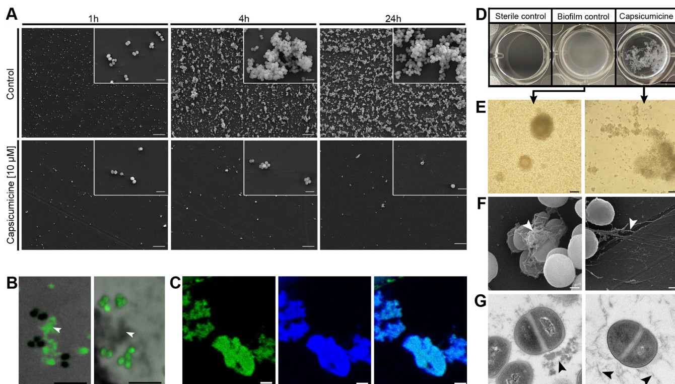
FIG 2 Biological characterization of capsicumine by microscopic approaches. (A) SEM images of polystyrene coupons after 1, 4, or 24 h of culture with Staphylococcus epidermidis (ATCC 35984). (Top) Peptide-less biofilm control. (Bottom) Cultures exposed to 10 μM capsicumine. Magnification \times 500 , with insets at \times 5,000 ; scale bars, 10 μm. (B) CFM images. (Left) S. epidermidis after exposure to 10 μM capsicumine-FITC with the peptide in green (fluorescence) and the bacterial cells in black (no fluorescence). (Right) Control, S. epidermidis after exposition to pseudonajide-FITC, an antibacterial peptide, this time showing the extracellular components in gray (no fluorescence). White arrows indicate extracellular content. Scale bars, 5 μm. (C) CFM images. S. epidermidis after exposure to 10 μM capsicumine-FITC (left) and after exposure to concanavalin A conjugates (selectively reveals saccharides) (center) and their colocalization (right). Scale bars, 5 μm. (D to G) The organizational state of S. epidermidis biofilm after 24 h in the presence (right) or absence (control, left) of capsicumine. (D) Macroscopic examination by pictures from the bottom of 24-well plates. The “sterile control” shows no bacteria or biofilm formation, the “biofilm control” shows homogenous adhered layers of bacteria, and “capsicumine” shows nonadhered bacteria but agglutinates. Scale bar, 5 mm. (E) TLM images show the biofilm control with overlapping attached bacterial clusters, while the capsicumine-exposed culture shows agglutinated nonadhered cells. Scale bar, 20 μm. (F) SEM images show the control with dense globular-like matrix features, while the capsicumine-exposed culture shows fibrillary branch-like oligomer structures. Scale bar, 200 nm. (G) TEM images of the biofilm control show denser assembled structures, while the capsicumine-exposed displays thin fibrillary oligomer structures. Scale bar, 200 nm. Arrows indicate the matrices.
