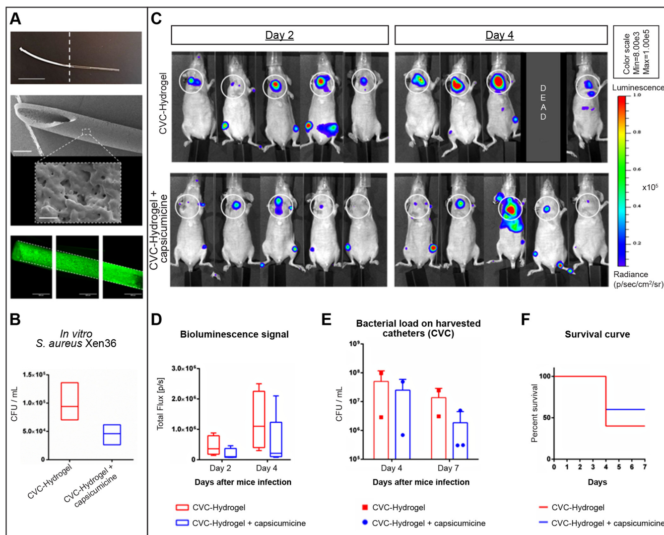
FIG 5 Assessment of capsicumine precoated central venous catheter (CVC) in mice (SKH1) infected by Staphylococcus aureus Xen36. (A and B) In vitro CVC development. (A) From the top to the bottom, a picture of up to half capsicumine precoated CVC (whitish) (scale bar, 1 cm), SEM image of precoated CVC (scale bar, 0.5 mm and its magnification scale bar, 1 \mu m), and a compilation of images of fluorescence microscopy of precoated CVC (capsicumine-FITC in green). (B) Bacterial load on CVC. (C to F) In vivo CVC assessment. (C) IVIS images (radiance thresholded and smoothed with a bidimensional Gaussian filter) of ventral position for each mouse at each time point. The control group (CVC-hydrogel) is shown in the top and the treated (CVC-hydrogel + capsicumine) in the bottom. White circles delimitate the CVC localization, and the luminescence scale is presented in radiance. (D) Bioluminescence quantification (ROI mean signals \pm standard deviation [SD]) is shown as photons total flux (p/s) for each group at each time point. (E) Bacterial load (CFU/ml) on harvested CVC for each mouse at each time point (day 4 and 7 after infection). (F) The Kaplan-Meier survival curve (% of survival) at each group during the 7 days after infection. All bioluminescence data and analyses were performed using IVIS Spectrum of Perkin Elmer. All experiments were conducted in accordance with ethical committee and the French authorities ( n = 5 /group). Bioluminescence images are presented with a defined pseudocolor scale to visualize the intensity of signals emitted.
