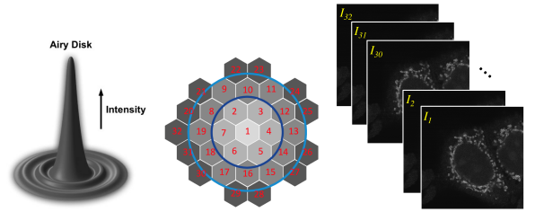
Fig. 1. Scheme of the array detector and image stack. The 32 sub-detectors are hexagonal and arranged around the central sub-detector. The dark blue (resp. light blue) circle highlights the group of N = 7 (resp. N = 19 ) central detectors. The detectors inside/outside the circles are called “inner”/“outer” detectors.
