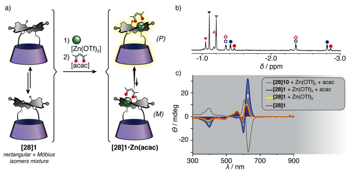
Fig. 5. (a) Metalation scheme of [28]1 with \text{Zn}(\text{OTf})_2 and \text{acac} in \text{CDCl}_3/\text{CD}_3\text{OD} (9:1) at room temperature. (b) Shielded region of the ^1\text{H} NMR spectrum of the metalation ( \nabla, \nabla, \nabla, \nabla : \text{CH}_3^{\text{acac}} introverted for the four isomers; \circ, \bullet, \circ, \bullet : inner \beta\text{CH} for the four isomers). (c) Electronic circular dichroism spectra of [28]1 after the sequential addition of \text{Zn}(\text{OTf})_2 and \text{acac} in \text{CDCl}_3/\text{CD}_3\text{OD} (9:1) at room temperature and ECD spectrum [28]10 metalated in the same conditions (intensity arbitrary scaled)[4d].
