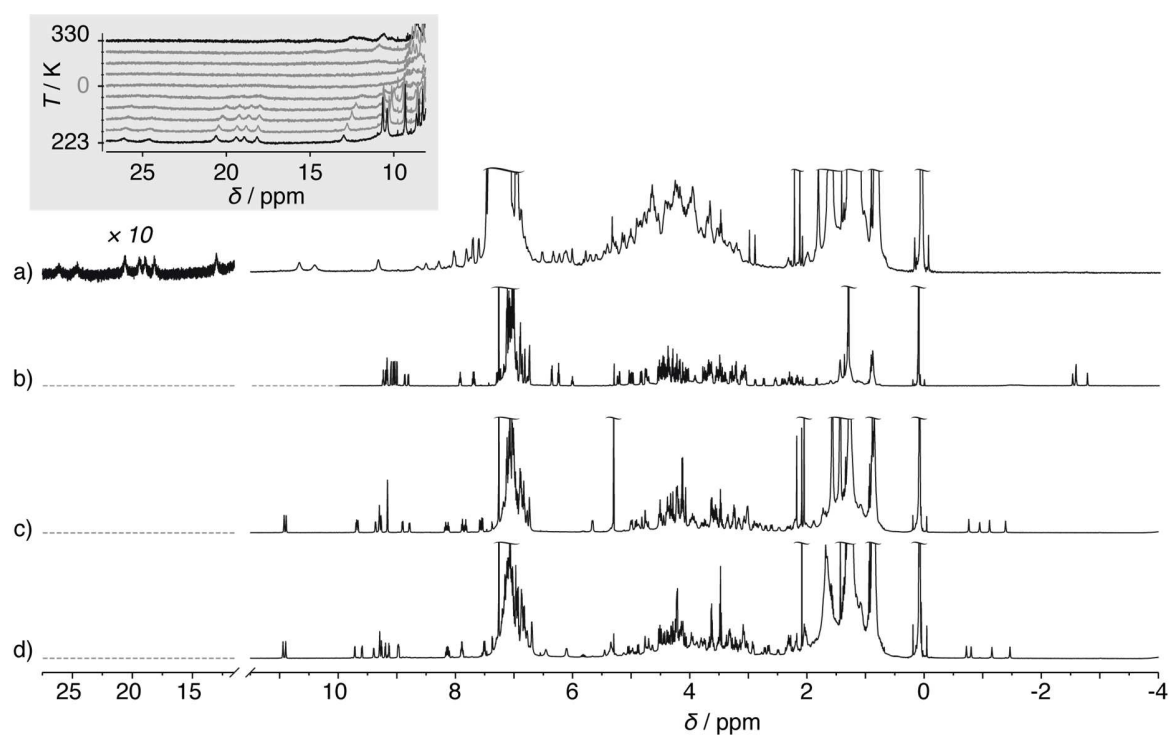
Fig. 3. (a) ^1\text{H} NMR (500 MHz) of [28]1 at 223 K in \text{CDCl}_3 (grey inset : VT-NMR of the deshielded region between 223 and 330 K). (b) ^1\text{H} NMR (600 MHz) of [26]1 at 340 K in \text{CDCl}_3 . (c) ^1\text{H} NMR (500 MHz) of [26]2a at 300 K in \text{CDCl}_3 . (d) ^1\text{H} NMR (500 MHz) of [26]2b at 300 K in \text{CDCl}_3 .
