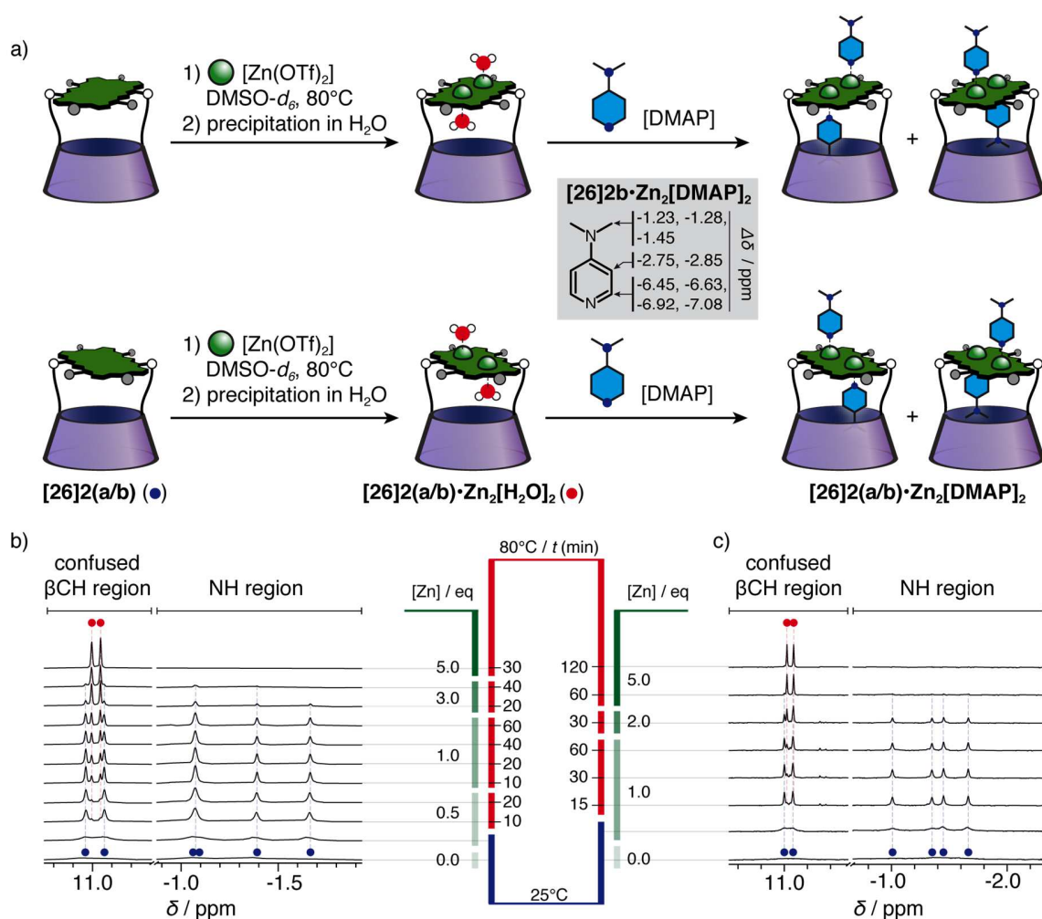
Fig. 6. (a) Metallation scheme of [26]2a and [26]2b with Zn(OTf)_2 in DMSO- d_6 at 80°C, followed by coordination of DMAP in CDCl_3 or CD_2Cl_2 at room temperature. (b) Stacked spectra of the ^1H NMR titration (500 MHz, DMSO- d_6 , 300K) of [26]2a with Zn(OTf)_2 (up to 5 equivalents; heating periods at 80°C are indicated for each amount of [Zn] ). (c) Stacked spectra of the ^1H NMR titration (500 MHz, DMSO- d_6 , 300K) of [26]2b with Zn(OTf)_2 (up to 5 equivalents; heating periods at 80°C are indicated for each amount of [Zn] ). Grey inset: complexation induced shifts ( \Delta\delta ) of the DMAP protons of [26]2b·Zn 2 [DMAP] 2 (measured at 210 K in CD_2Cl_2 ).
