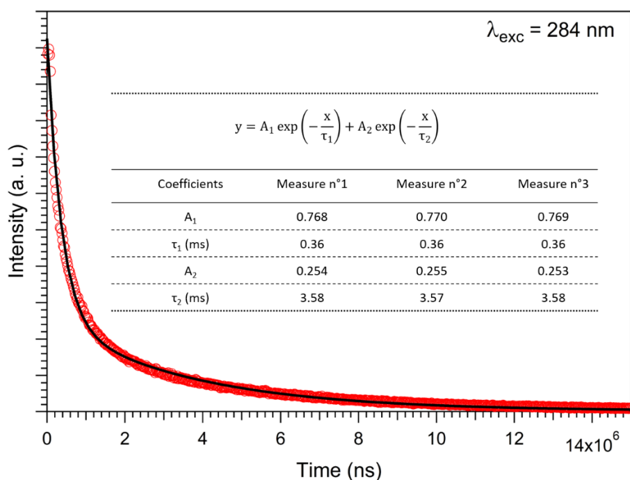
Figure S2. Luminescent decay measurement of Zn 0.98 Mn 0.02 CN 2 at 300 K under photo-excitation at 284 nm.
