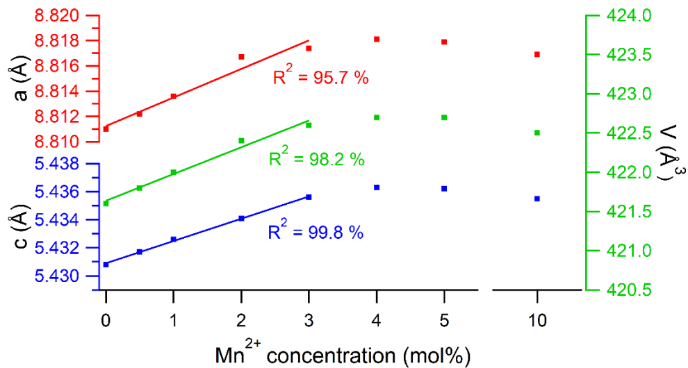
Figure 2. Evolution of the a , c unit cell parameters and V cell volume in \text{Zn}_{1-x}\text{Mn}_x\text{CN}_2 samples as a function of \text{Mn}^{2+} doping concentration.
