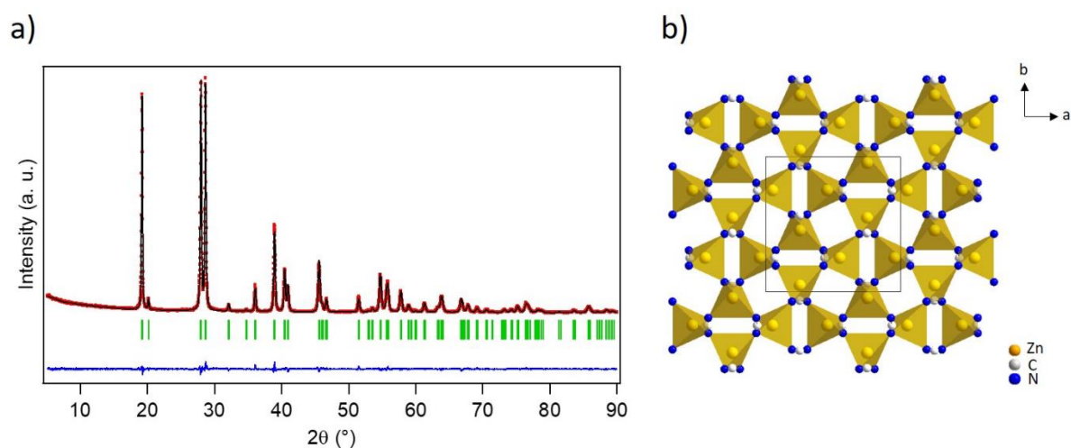
Figure 1. a) Final Rietveld refinement pattern for \text{Zn}_{0.98}\text{Mn}_{0.02}\text{CN}_2 : observed (red dotted line), calculated (black full line) and difference (blue line) X-ray powder diffraction profiles from the pattern-matching plot obtained with Fullprof. The vertical markers correspond to the position of the Bragg reflections. b) Crystal structure of \text{ZnCN}_2 .
